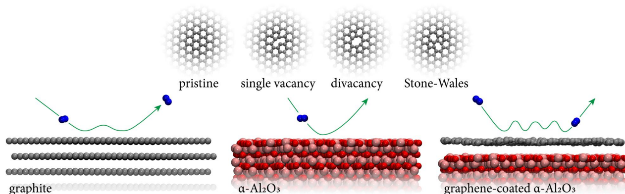
FIG. 1. Schematic representation of the simulated systems. Nitrogen molecule impinging on the multilayer graphite surface, the \alpha\text{-Al}_2\text{O}_3 (0001) slab, and the graphene-coated \alpha\text{-Al}_2\text{O}_3 (0001) surface. The inset shows the pristine graphene lattice and the optimized atomic configurations of the key defects studied: single vacancy, divacancy, and Stone–Wales defect.
