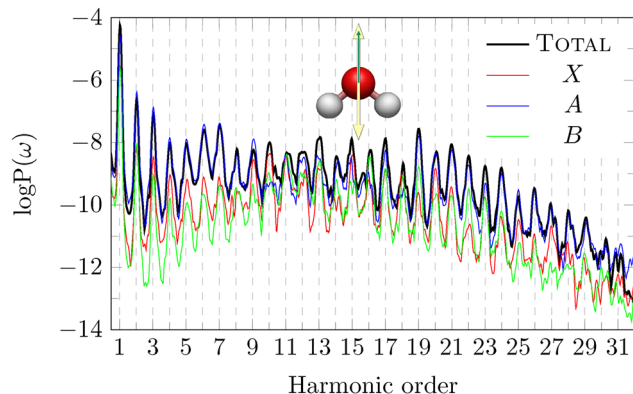
Fig. 4 Total and partial HHG spectra of H 2 O, with pulse polarisation parallel to the principal axis ( z axis). This system corresponds to the configuration (c) of Fig. 2. The yellow double arrow represents the pulse polarisation, while a green arrow represents the direction of detection of the HHG signal.
