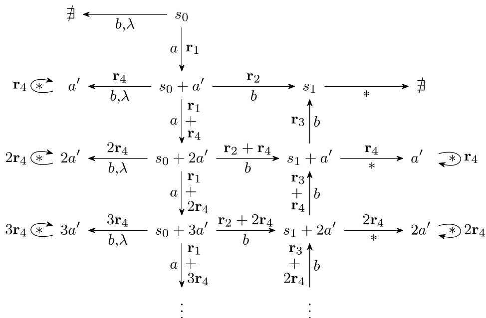
Fig. 4 Schematic representation of all possible processes of the chemical pure reaction automaton of Example 3, which accepts the language \{a^n b^n \mid n > 0\} .
