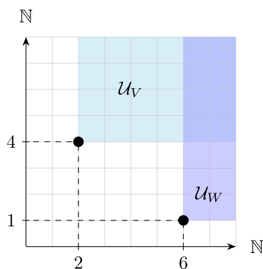
Fig. 1 Visual representation, under the isomorphism of Remark 2, of the open sets corresponding to V = 2a + 4b \mapsto (2, 4) \in \mathbb{N}^2 and W = 6a + b \mapsto (6, 1) \in \mathbb{N}^2
