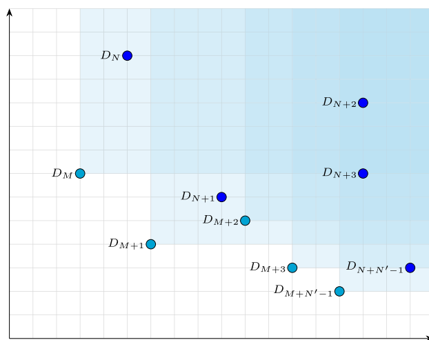
Fig. 3 Example of multisets \{D_M, D_{M+1}, \dots, D_{M+N'-1}\} whose corresponding open sets bound the dynamics of the automaton
