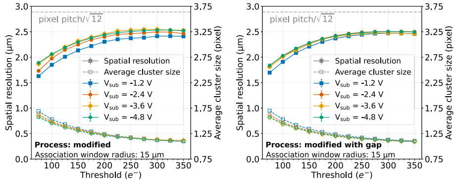
Fig. 9. Spatial resolution and cluster size as a function of the applied threshold for the modified (left) and modified with gap (right) structures, comparing different reverse substrate voltages in different colors. The gray dashed line represents the pixel pitch divided by \sqrt{12} .
