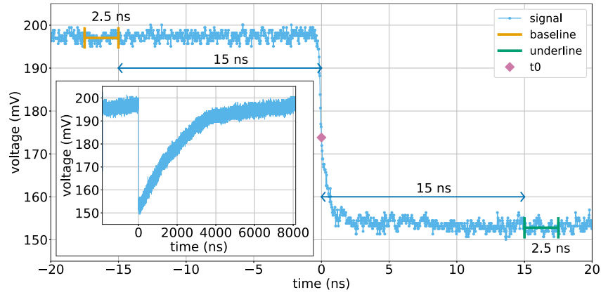
Fig. 6. Typical signal acquired by the oscilloscope with baseline, underline, and t_0 definitions. The x-axis is shifted to put t_0 at the origin to highlight the time intervals for the baseline and underline definitions.
