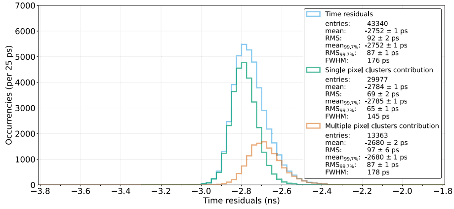
Fig. 13. Distributions contributing to non corrected time residuals (blue histogram) divided according to the associated cluster size for the DUT implementing modified with gap process operated at V_{\text{sub}} = -4.8 V. The green distribution represents the time residual values related to single pixel clusters, while the red one describes the contribution of clusters with pixel multiplicity larger than one.
