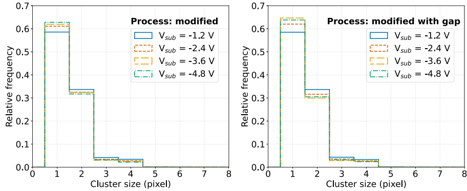
Fig. F.21. Cluster size distribution of the APTS-OA modified and modified with gap DUT at 100 e^- threshold at different V_{sub} = V_{pwell} configurations.
