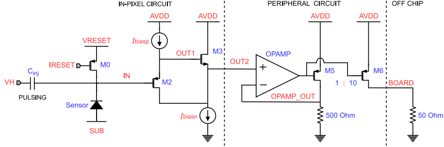
Fig. 3. Left: APTS-OA front-end circuit with the circuitry inside the pixel. Right: circuitry located in the periphery of the matrix. The off chip line to the measurement system is also represented.
