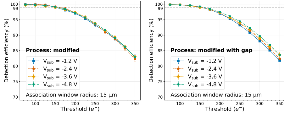
Fig. 8. Detection efficiency for the modified (left) and modified with gap (right) pixel processes as a function of the applied threshold and for different V_{\text{sub}} . The dashed line in both plots indicates the 99% detection efficiency.
