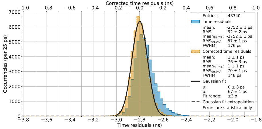
Fig. 10. Time residuals measured for the modified with gap process DUT operated at V_{\text{sub}} = -4.8 V, before (blue distribution, bottom horizontal axis) and after (orange distribution, top horizontal axis) time walk-like correction. The latter distribution is fitted with a Gaussian function on a range of \pm 3\sigma (black solid line, dashed line for points outside the fit range).
