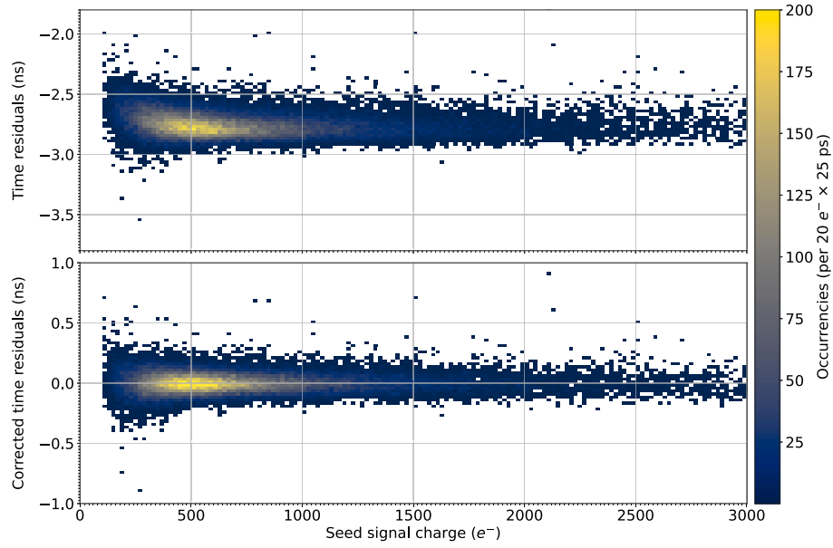
Fig. 11. Time residuals versus seed signal charge with no correction applied (top) and after the correction (bottom) for the DUT featuring modified with gap process operated at V_{\text{sub}} = -4.8 V.
