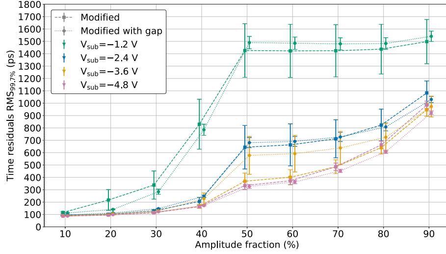
Fig. D.19. Time residuals distribution width for APTS-OA DUTs' signal times measured at different fractions of the signal amplitude for each operation V_{sub} . The values pertaining to the modified process DUT are indicated with square markers and dashed lines, while those referring to the modified with gap process DUT with circle markers and dotted lines. A slight displacement in the x axis is added between the two curves to allow better visibility.
