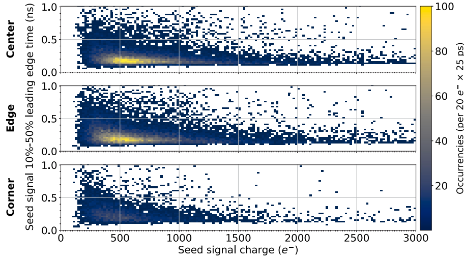
Fig. G.22. Correlation between seed signal charge and signal leading edge time for the APTS-OA modified with gap DUT operated at V_{\text{sub}} = -4.8 V. Data is grouped in three different datasets depending on the reconstructed in-pixel track hit position.
