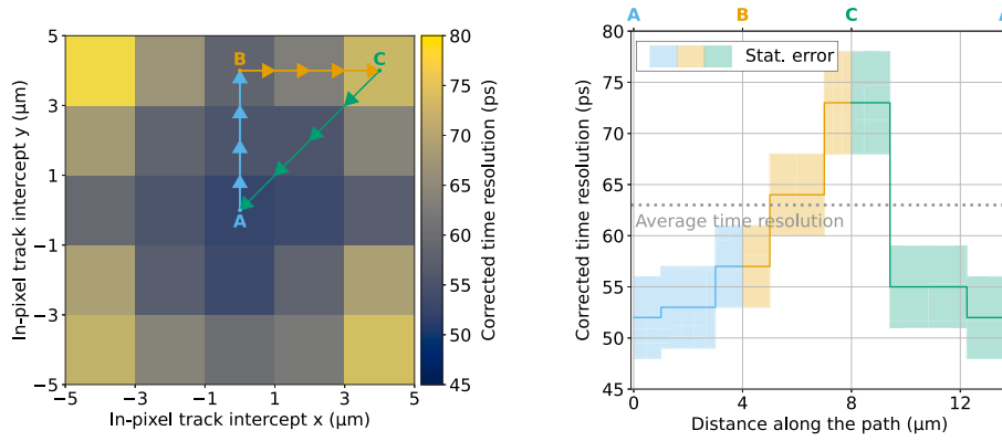
Fig. 15. Left: corrected in-pixel time resolution of the modified with gap structure operated at V_{\text{sub}} = -4.8 V. Right: time resolution variation along the path from the pixel center to the edge, and to the corner.
