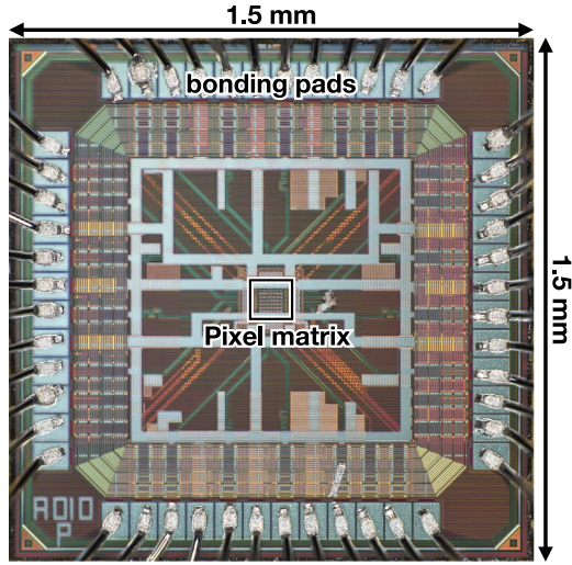
Fig. 1. Photograph of the APTS-OA taken with a microscope.
