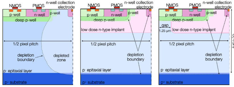
Fig. 2. Schematic cross section of the three pixel process variants of the APTS. From left to right: standard, modified featuring a low dose deep n-type implant, and modified with gap employing a low dose deep n-type implant with a gap at the pixel's edges. Not to scale. [13].
