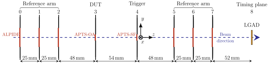
Fig. 5. Schematic of the test beam setup showing each detector plane.
