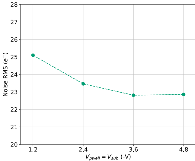
Fig. C.17. Noise RMS of the APTS-OA modified with gap at different V_{\text{sub}} = V_{\text{pwell}} configurations.
