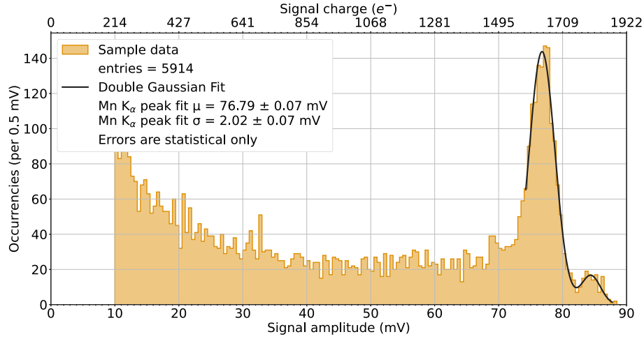
Fig. 7. Amplitude distribution of signals acquired with the ^{55}\text{Fe} source for a single pixel read out with the oscilloscope. The ^{55}\text{Mn-K}_\alpha and \text{K}_\beta peaks are fitted together with the sum of 2 Gaussian functions.
