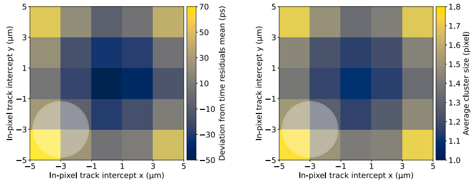
Fig. 12. Map of the deviation from the time residuals mean value (left) and cluster size map (right) for in-pixel track incidence positions for the DUT based on modified with gap process operated at V_{\text{sub}} = -4.8 V. The tracking resolution is represented by the white circle ( r = \sigma_{\text{track}} = 1.8 \mu\text{m} ) in the bottom left corner of both maps.
