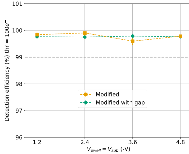
Fig. E.20. Detection efficiency of the APTS-OA modified and modified with gap DUT at 100 e^- threshold at different V_{sub} = V_{pwell} configurations.
