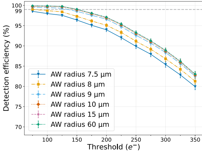
Fig. B.16. Detection efficiency of the APTS-OA modified DUT as a function of the threshold at V_{\text{sub}} = V_{\text{pwell}} = -1.2 V, varying the association window (AW) radius.
