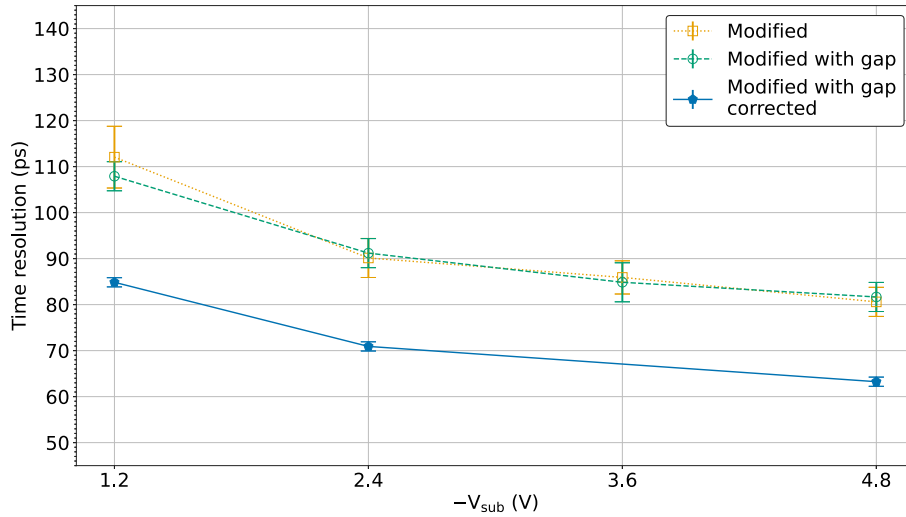
Fig. 14. Non-corrected (open symbols, orange dotted line and green dashed line) and corrected (full symbols, blue solid line) time resolution measured for modified and modified with gap DUT process variants. A time walk-like correction, described in Section 3.2, is applied only to high statistical significance data sets, namely those measured with the modified with gap structure.
