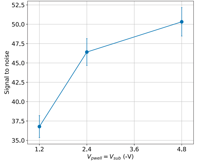
Fig. C.18. Signal to noise of the APTS-OA modified with gap at different V_{\text{sub}} = V_{\text{pwell}} configurations.
