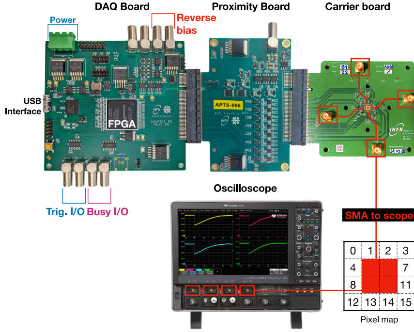
Fig. 4. Scheme of the APTS-OA readout system. From left to right: picture of the DAQ board, hosting the firmware control FPGA as well as trigger, busy, and reverse bias connection, the proximity board, hosting ADCs for external pixel readout, and the carrier board to which the chip is glued and wire bonded. In the bottom part, a sketch of the 4 \times 4 pixel matrix with the four inner pixels (highlighted in red) connected to an oscilloscope.
