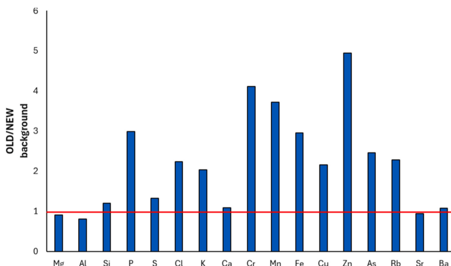
Fig. 4. Ratios between background values of PTEs accumulated by OLD and NEW samples. The red line indicates 1 (no change). (For interpretation of the references to colour in this figure legend, the reader is referred to the Web version of this article.)
