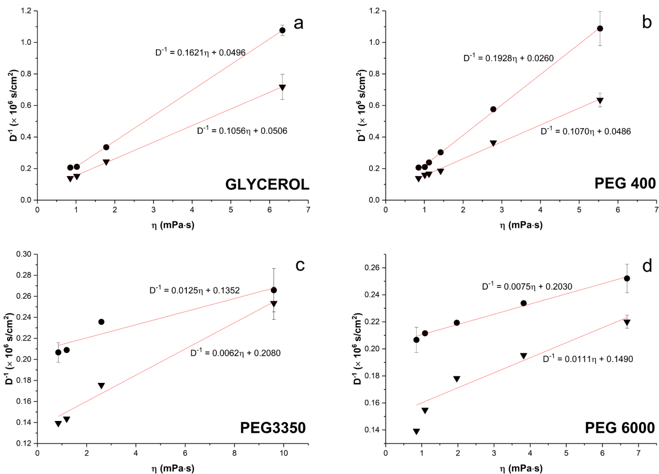
Fig. 6. Reciprocal diffusivity ( D^{-1} ) of CAF (▼) and HC (●) as a function of diffusion media viscosity ( \eta ) for: a) glycerol, b) PEG400, c) PEG3350 and d) PEG6000. Red lines show linear regression fitting to the experimental data according to Eq. (13) (fitting parameters summarized in Supplementary material). Error bars show SD ( n = 3 ).
