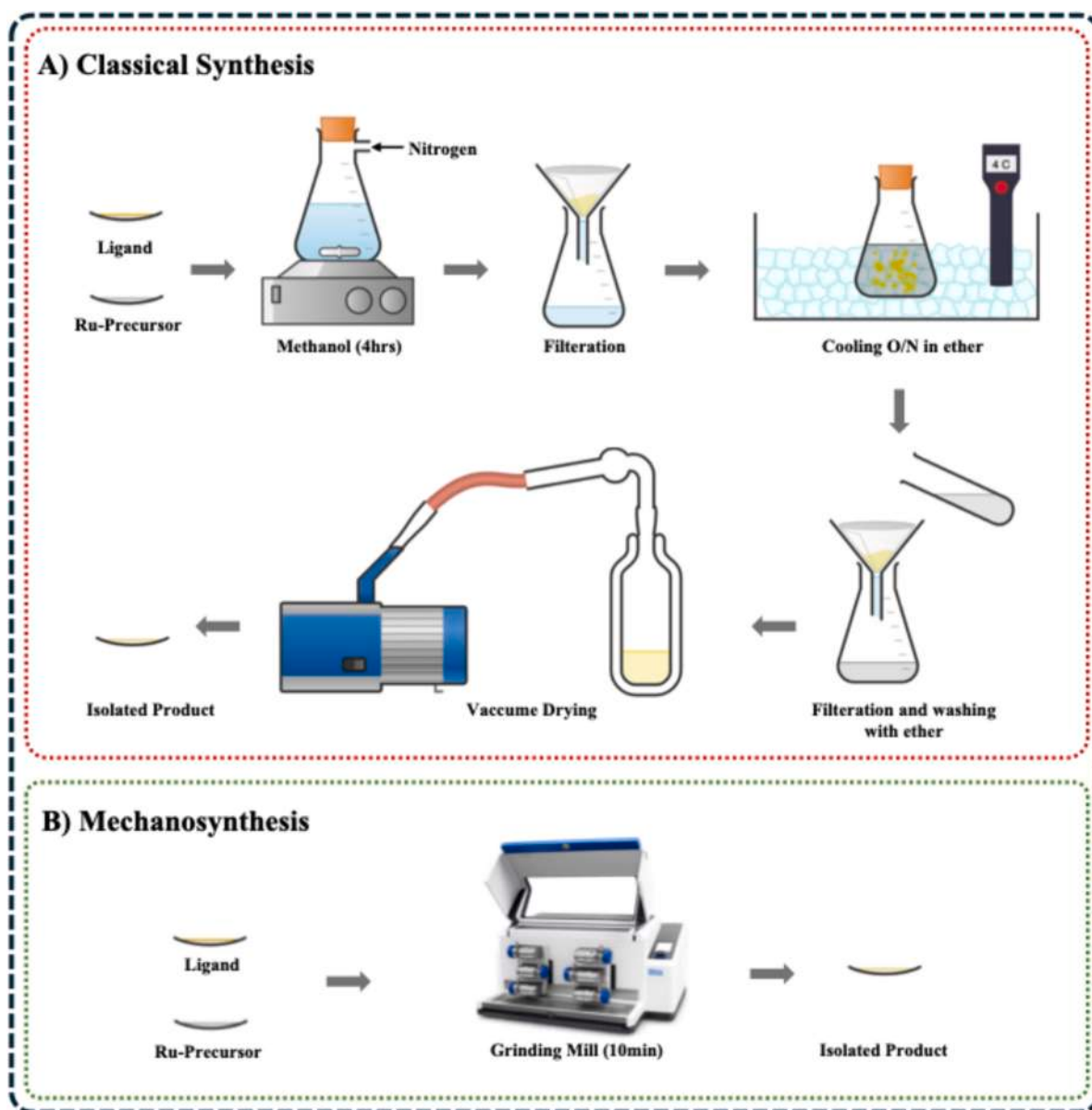
Fig. 2. Comparison of Classical solution based synthesis [121] with Mechanochemistry [95] of [\text{Ru}(\text{p-Cym})(\text{BiPy})\text{Cl}]\text{Cl}(\mathbf{29}) .
