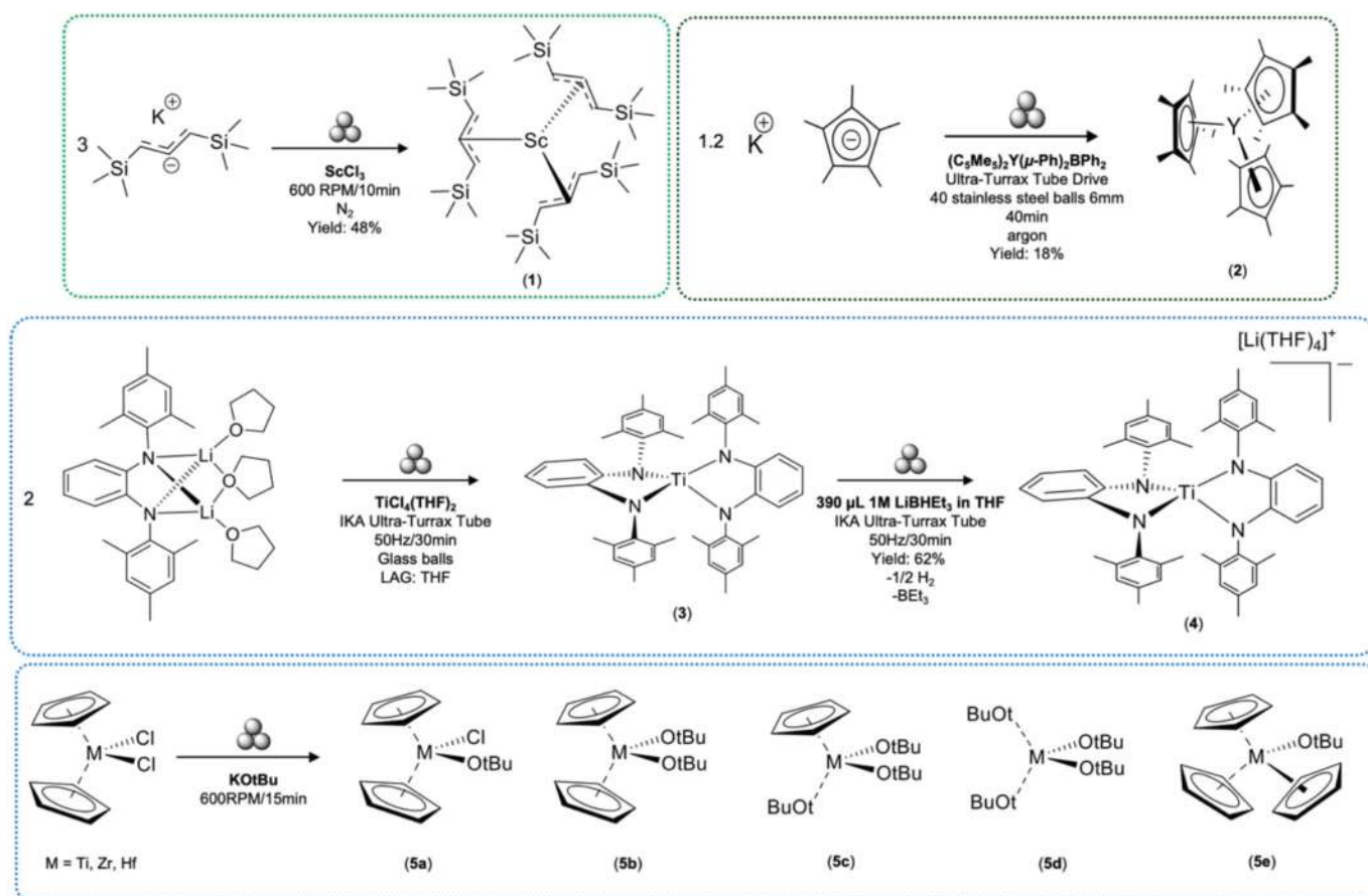
Scheme 1. Summary of Sc(III), Y(III), Ti(III/IV), Zr(IV) and Hf(IV) complexes prepared by mechanochemical synthesis.
