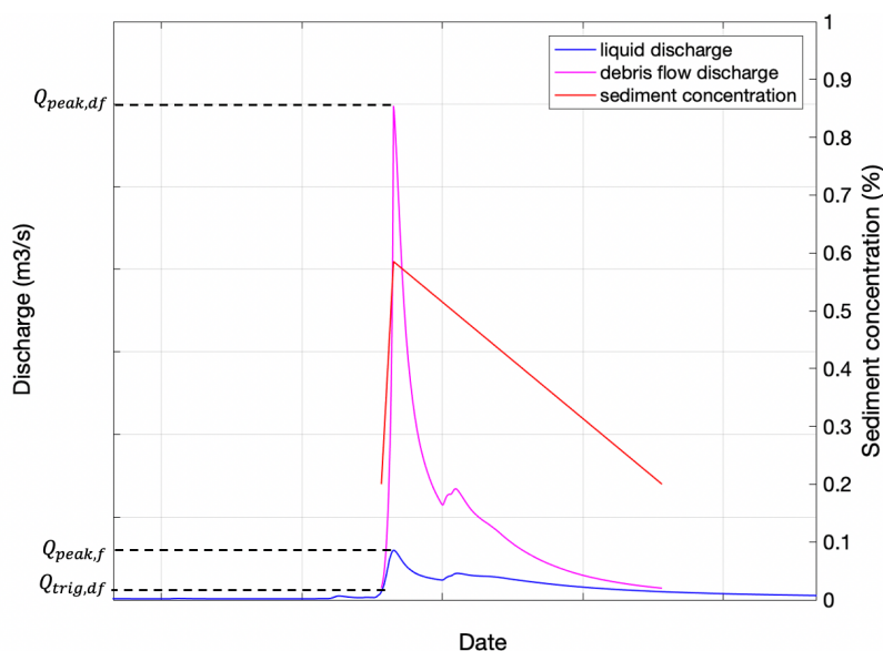
Figure 2. Debris-flow hydrograph that can be obtained according to the Takahashi (1991) revised by D’Agostino and Marchi (2003).
