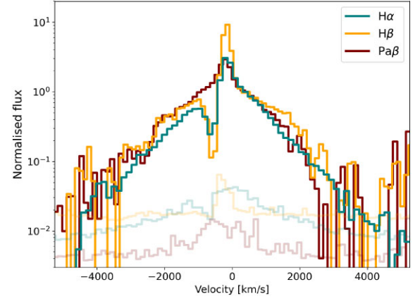
Figure 1. Line profile comparison in velocity space and on logarithmic scale for H\alpha , H\beta , and \text{Pa}\beta . Their fluxes are normalized to the red 500 \text{ km s}^{-1} . Spectral errors are reported in lighter colours.
