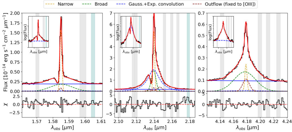
Figure 2. Best-fitting models for H \beta (left), H \alpha (centre), and Pa \beta (right). Individual model components are reported in different colours; each line is decomposed into three Gaussians (narrow, outflow, and broad unscattered components) and the exponential convolution representing the broad scattered component. For the H \beta and H \alpha , the absorber is also modelled. The three inset panels report the line profiles in logarithmic scale, with the best-fitting model in red and the exponential component in blue. Shaded regions indicate the locations of possible He I (light blue) and [Fe II] (light grey) lines.
