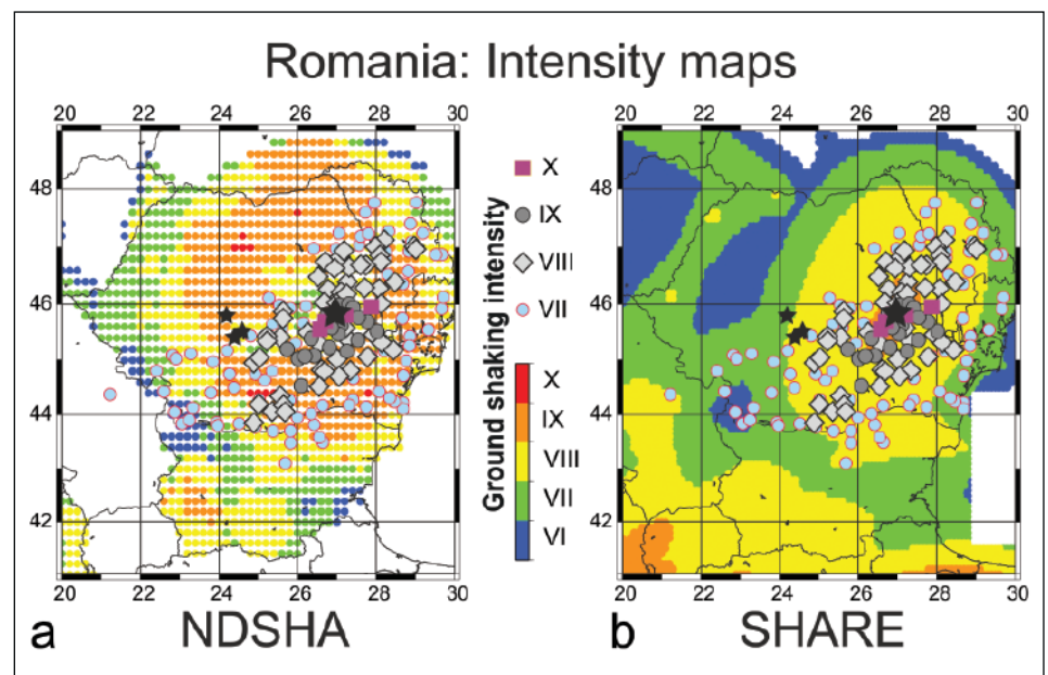
Fig. 1. Seismic hazard assessment for Romania. (a) Neodeterministic seismic hazard assessment (NDSHA) method [Radulian et al. , 2000]; (b) Seismic Hazard Harmonization in Europe (SHARE) project [Giardini et al. , 2014]. Colored regions represent shaking intensities calculated using each method. Color-coded symbols indicate observed shaking intensities. The large star marks the shock epicenter of the 1940 M7.7 earthquake in Vrancea, and smaller stars are epicenters of violent shocks in the Fagaras zone in 1550, 1571, and 1590.
