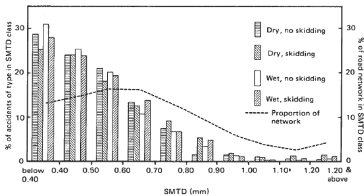
Fig. 4. Relationship between macrotexture at crash sites and skid resistance at all sites on Network C
