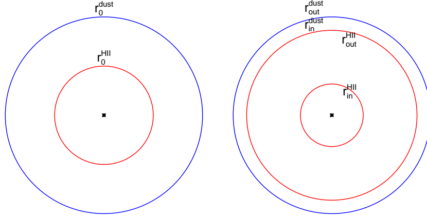
Fig. A.1. Sketch of the adopted spherical configuration. Left : the initial state, with uniform density and magnetic field; there are no separate ionized and dust shells. Right : present-day state with a cavity inside r_{in}^{HII} , an ionized shell between r_{in}^{HII} and r_{out}^{HII} , and a dust shell between r_{in}^{dust} = r_{out}^{HII} and r_{out}^{dust} . The present-day radii r_{in}^{HII} , r_{out}^{HII} , and r_{out}^{dust} correspond to initial radii 0, r_0^{HII} , and r_0^{dust} , respectively.
