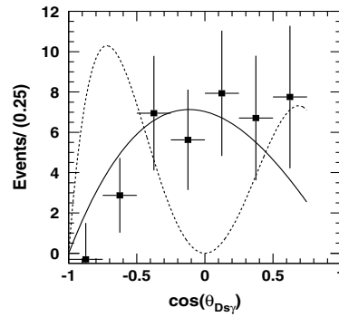
Figure 19.3.21. From (Krokovny, 2003b): Background-subtracted helicity distribution for the D_{s1}(2460)^+ \rightarrow D_s^+\gamma . Lines show MC expectations for spin hypotheses J = 1 (solid) and J = 2 (dashed); J = 0 is forbidden.
