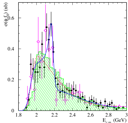
Figure 21.3.14. The e^+e^- \rightarrow \phi f_0(980) cross sections measured in the K^+K^-\pi^+\pi^- (circles) and K^+K^-\pi^0\pi^0 (squares) final states using an integrated luminosity of 232 fb -1 by BABAR (Aubert, 2007bc). The hatched histogram shows the simulated cross section in the no-resonance hypothesis, which is consistent with a fit to the data with only a non-resonant component (dashed line). The solid line represents the result of the fit described in the text assuming the presence of the Y(2175) .
