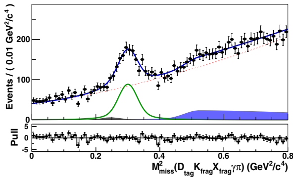
Figure 19.1.7. From (Zupanc, 2013b). M_{miss}^2(D_{tag}KX_{frag}\gamma\pi) distribution of partially reconstructed D_s^+ \rightarrow \eta\pi^+ decays within the inclusive D_s sample. The fit result is superimposed and includes fitted signal contribution (solid green line), reflections from charged pion originating from D_s^+ \rightarrow K^0\pi^+ (full grey histograms) and other true D_s decays ( D_s^+ \rightarrow \rho K^+ \rightarrow \pi^+\pi^-K^+ and D_s^+ \rightarrow \bar{K}^0 K^+ due to K - \pi mis-reconstruction) (full blue histogram), and combinatorial background (dashed red line).
