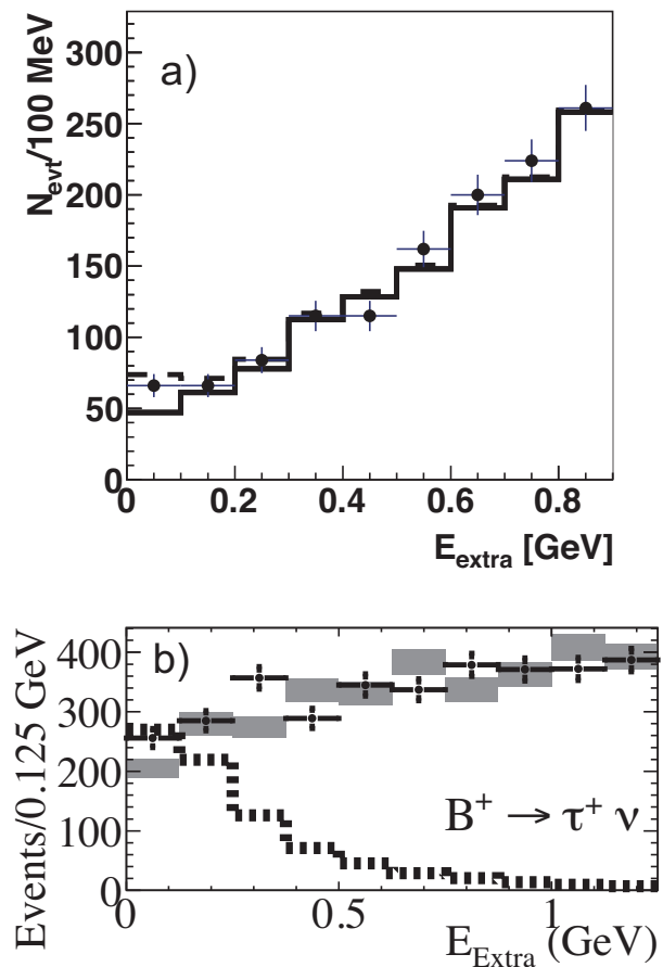
Figure 17.10.3. (a) Distribution of E_{\text{extra}} reported by BABAR using hadronic tags (Lees, 2013a). The points with error bars represent data. The solid histogram shows the background and the dashed component is the best-fit signal excess distribution. (b) The same distribution obtained using semileptonic tagged events (Aubert, 2010a). The points with error bars are data. The gray shaded boxes represent MC simulated backgrounds and the dotted histogram is the signal MC simulation normalized to 10 times the expected branching fraction.
