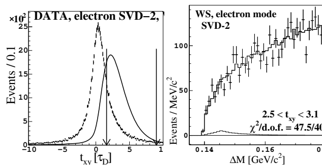
Figure 19.2.23. Left: The distribution of the decay time in the transverse plane for selected WS events (dots). The solid line shows the simulated distribution of signal events and the vertical arrows the interval selected for the signal. Right: An example of the fit to the \Delta M data distribution (points) in a single t_{xy} bin for the WS e - 2 data subsample. The histogram is the fit to the distribution, with the contribution of signal shown along the horizontal axis. From (Bitenc, 2008).
