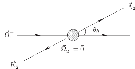
b) All decay products in the \Omega^- rest-frame; in this frame, \bar{\Omega}_1^- \rightarrow \bar{\Omega}_2^- = \vec{0}, \bar{\Lambda}_1 \rightarrow \bar{\Lambda}_2, \bar{K}_1^- \rightarrow \bar{K}_2^- .
