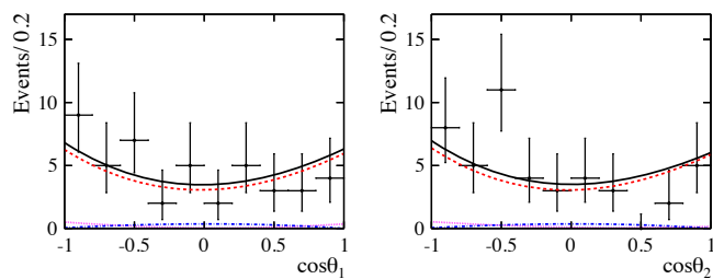
Figure 23.3.7. Helicity angle distributions and projections of the fit result for B_s^0 \rightarrow D_s^{*+} D_s^{*-} . The red dashed (blue dash-dotted) curves show the transverse (longitudinal) components; the magenta dotted curves show background; and the black solid curves show the total. Plots are from Esen (2013).
