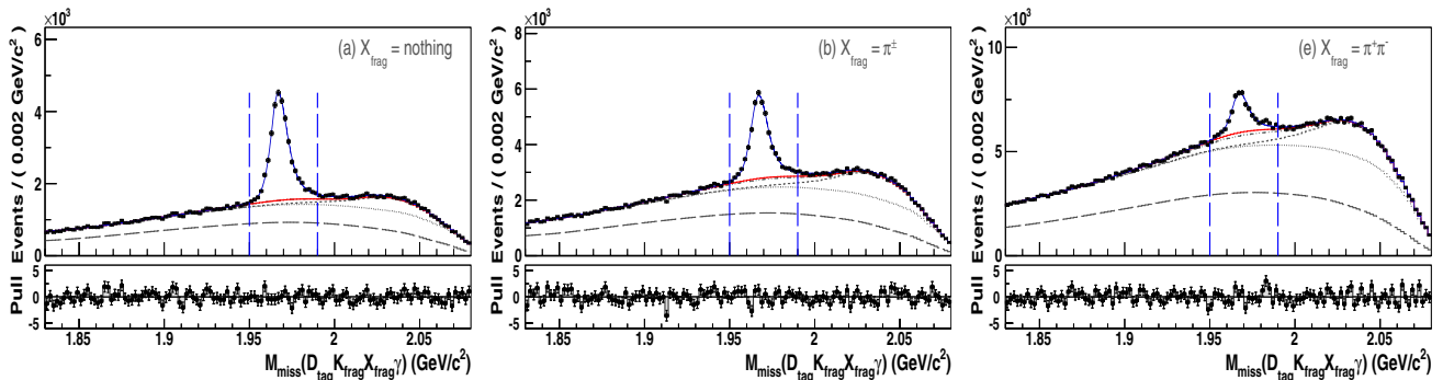
Figure 19.1.4. From (Zupanc, 2013b). Inclusive D_s in M_{miss}(D_{tag} K X_{frag} \gamma) for three out of seven possible X_{frag} modes. The solid blue (red) line shows the contribution of signal and background (background only) candidates. The cumulative contributions of candidates originating from different background sources as described in the text are shown with different gray dashed lines. Dashed vertical lines indicate the signal region considered in further analysis.
