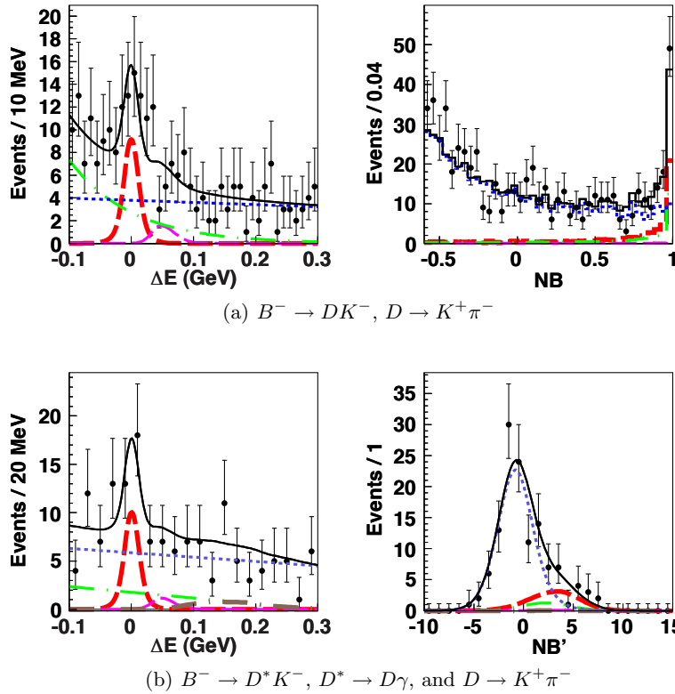
Figure 17.8.4. \Delta E and neural-network NB (or NB' , a modified NB variable) distributions in a signal-enriched region for B^- \rightarrow DK^- where D \rightarrow K^+\pi^- (top; Horii, 2011) and for B^- \rightarrow D^*K^- where D^* \rightarrow D\gamma and D \rightarrow K^+\pi^- (bottom; Trabelsi, 2013) from the Belle collaboration. In these plots, DK^- components are shown by thicker dashed curves (red), and D\pi^- components are shown by thinner curves (magenta). B\bar{B} backgrounds are shown by dash-dotted curves (green) while q\bar{q} backgrounds are shown by dotted curves (blue). The sum of all components are shown by solid curves (black).
