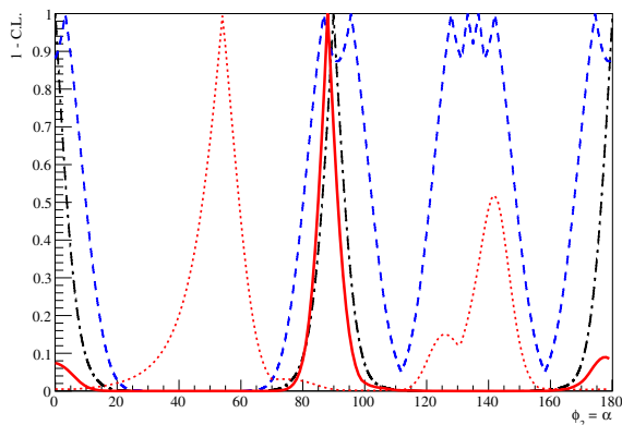
Figure 17.7.14. The 1 - \text{C.L.} function obtained on \phi_2 = \alpha from the B Factories (solid thick red curve). Constraints obtained using the Gronau-London isospin analysis for (dashed blue) B \rightarrow \pi\pi and (dash-dotted black) \rho\rho decays as well as the Dalitz analysis for (dotted red) \pi^+\pi^-\pi^0 decays are shown.
