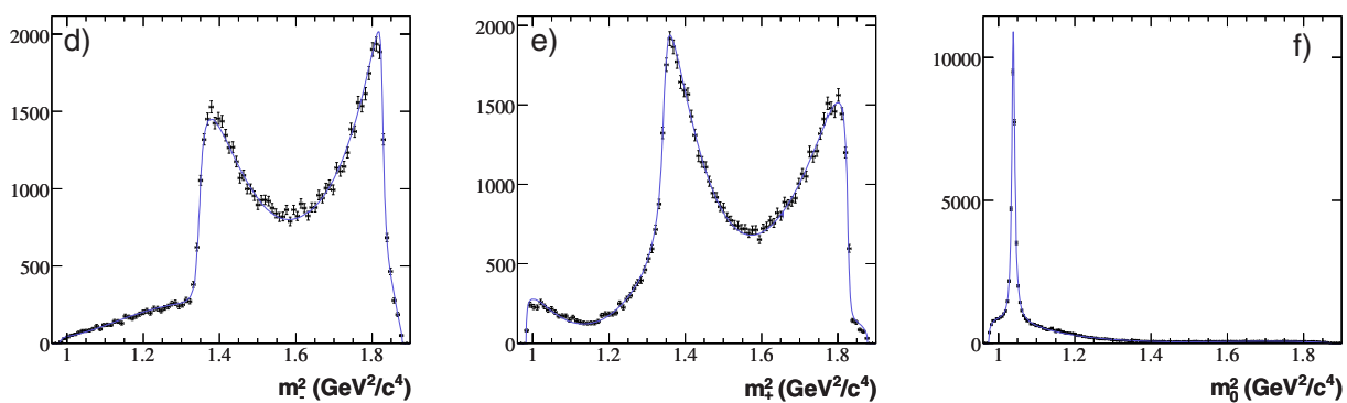
Figure 19.1.21. From (Aubert, 2008l). D^0 \rightarrow K_s^0 K^+ K^- Dalitz plot projections from D^{*+} \rightarrow D^0 \pi^+ events on (d) m_-^2 , (e) m_+^2 , and (f) m_0^2 . The curves are the reference model fit projections.
