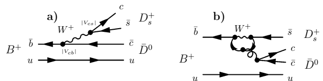
Figure 17.3.3. Spectator a) and penguin b) diagrams contributing to B^+ \rightarrow D_s^+ D .
