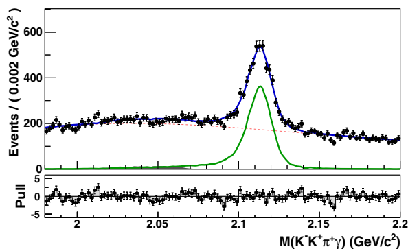
Figure 19.1.5. From (Zupanc, 2013b). M(K^+ K^- \pi^+ \gamma) mass distribution of exclusively reconstructed D_s^+ \rightarrow K^+ K^- \pi^+ decays within the inclusive D_s sample, with the fit result superimposed and including fitted signal contribution (solid green line), reflection from D_s^* \rightarrow D_s \pi^0 \rightarrow K^+ K^- \pi^+ \gamma \gamma with one of the photons missing (full dark gray histogram) and combinatorial background (dashed red line).
