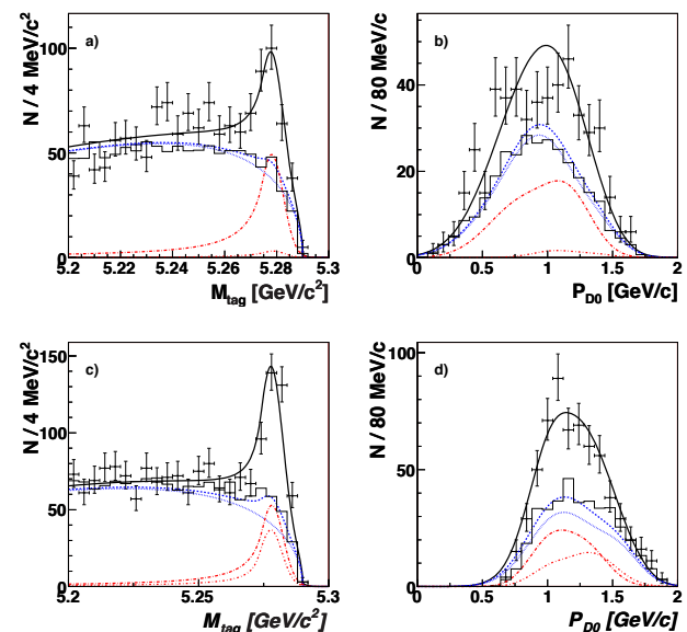
Figure 17.10.8. The fit projection to M_{\text{tag}} and p_{D^0} for M_{\text{tag}} > 5.26 \text{ GeV}/c^2 (a, b) for \bar{D}^{*0}\tau^+\nu_\tau and (c, d) for \bar{D}^0\tau^+\nu_\tau , from (Bozek, 2010).
