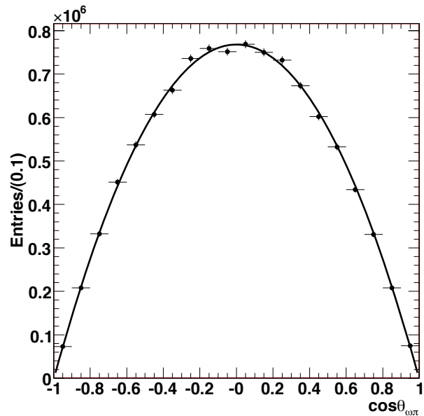
Figure 20.6.10. Distribution of \cos\theta_{\omega\pi} from \tau \rightarrow \omega(782)\pi^-\nu_\tau events in BABAR (Aubert, 2009ap). Here \theta_{\omega\pi} is the angle, in the \omega\pi^- rest frame, between the normal to the \omega \rightarrow \pi^+\pi^-\pi^0 decay plane and the direction of the pion. The curve shows a fit to determine the relative contributions from first-class and second-class currents.
