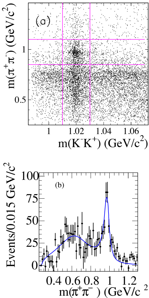
Figure 21.3.13. (a) The reconstructed m(\pi^+\pi^-) vs m(K^+K^-) distribution for the e^+e^- \rightarrow K^+K^-\pi^+\pi^- reaction measured by BABAR (Aubert, 2006c). The vertical lines identify the selected region around the \phi mass peak. (b) Background subtracted m(\pi^+\pi^-) distribution of selected e^+e^- \rightarrow \phi(1020)\pi^+\pi^- events (Aubert, 2007bc). The solid line is the results of the fit to the data with a coherent sum of two Breit-Wigner functions, referring to the f_0(600) and f_0(980) .
