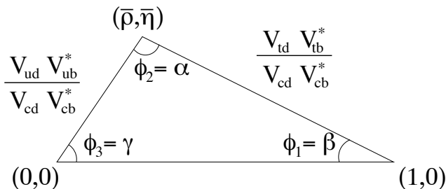
Figure 16.5.1. The Unitarity Triangle.
