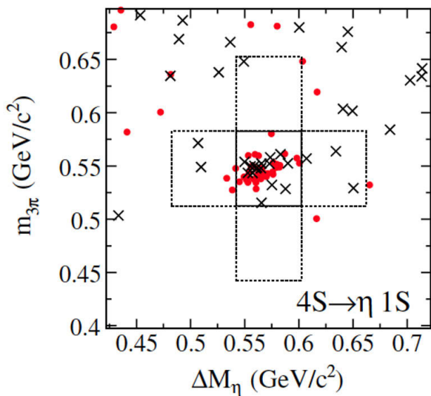
Figure 18.4.20. The distribution of M_{3\pi} vs \Delta M_\eta = M_{3\pi\ell\ell} - M_{ll} for \eta\Upsilon(1S) candidate events, demonstrating the observed signal (Aubert, 2008bc). Solid lines delimit the signal region, while dashed lines delimit the sideband regions used for the background estimate. Crosses represent the data from the \Upsilon(1S) \rightarrow e^+e^- sample and dots the data from the \Upsilon(1S) \rightarrow \mu^+\mu^- sample.
