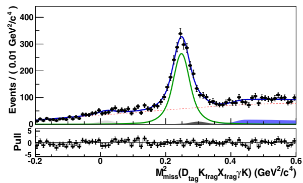
Figure 19.1.6. From (Zupanc, 2013b). M_{miss}^2(D_{tag} K X_{frag} \gamma K) distribution of partially reconstructed D_s^+ \rightarrow \bar{K}^0 K^+ decays within the inclusive D_s sample. The fit result is superimposed and includes fitted signal contribution (solid green line), reflections from charged kaon originating from D_s^+ \rightarrow \eta K^+ and D_s^+ \rightarrow \pi^0 K^+ (full grey histograms) and other true D_s decays (for example D_s^+ \rightarrow \eta \pi^+ with pion being misidentified as kaon) (full blue histogram), and combinatorial background (dashed red line).
