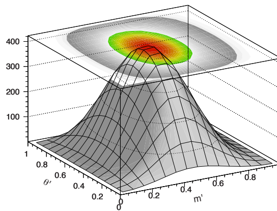
Figure 13.4.1. Jacobian determinant, Eq. (13.4.4), of the transformation, Eq. (13.4.1), defining the square Dalitz plot (SDP). Such a distribution would be obtained in the SDP if events were uniformly distributed over the nominal Dalitz plot.
