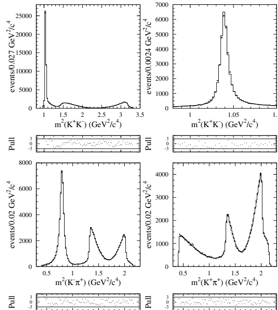
Figure 19.1.35. From (del Amo Sanchez, 2011b). D_s^+ \rightarrow K^+K^-\pi^+ : Dalitz plot projections. The data are represented by points with error bars, the fit results by the histograms. The upper right plot shows zoom of the m^2(K^+K^-) in the \phi mass region.
