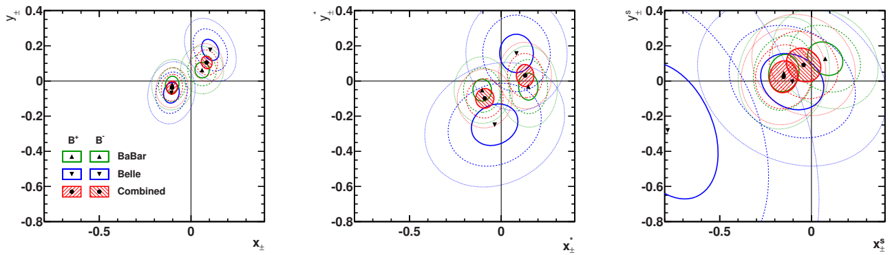
Figure 17.8.7. Contours at the 60.7% confidence level for 2 degrees of freedom (corresponding to -2\Delta \ln L = \Delta \chi^2 = 1 , i.e. , one standard deviation in two dimensions assuming Gaussian errors, solid lines), and two- and three-standard deviation contours (dashed lines) in the (left) z_{\pm} , (center) z_{\pm}^* , and (right) z_{\pm}^s planes, for BABAR and Belle separately (including all errors other than model uncertainties), and their HFAG combination (Asner et al., 2011).
