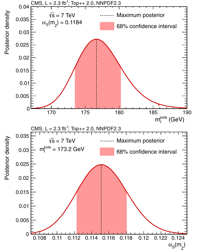
Fig. 3. Marginal posteriors P(m_t^{\text{pole}}) (top) and P(\alpha_s) (bottom) based on the cross section prediction at NNLO + NNLL with the NNLO parton distributions from NNPDF2.3. The posteriors are constructed as described in the text. Here, P(m_t^{\text{pole}}) is shown for \alpha_s(m_Z) = 0.1184 and P(\alpha_s) for m_t^{\text{pole}} = 173.2 GeV.
