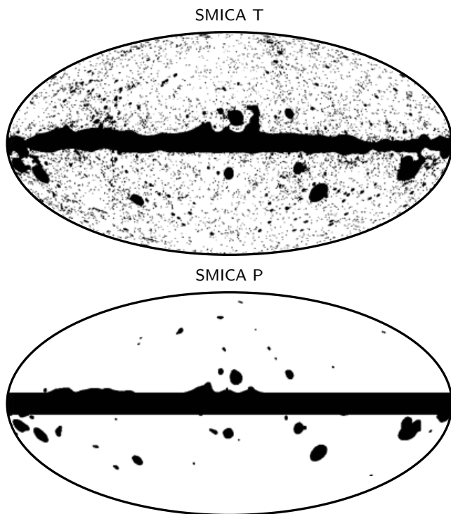
Fig. D.2. SMICA masks in temperature ( top ) and polarization ( bottom ).
