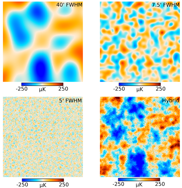
Fig. A.3. 5° × 5° zoom-in of the multi-resolution contributions to the Commander hybrid CMB map from the 40' (top left), 7.5' (top right) and ≈5' (bottom left) solutions, centered on the South Galactic Pole. The hybrid map is shown in the bottom right panel.
