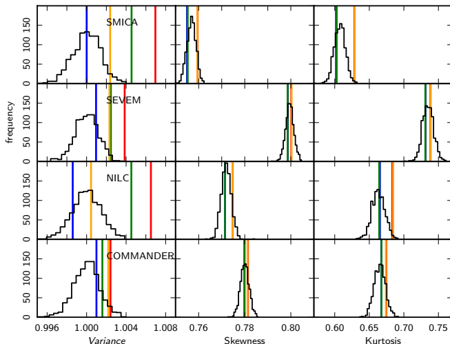
Fig. 16. Polarized intensity variance ( left column ), skewness ( middle column ), and kurtosis ( right column ) evaluated from the FFP8 Monte Carlo simulations (histogram) and from components of the fiducial FFP8 map at N_{\text{side}} = 1024 outside the FFP8-UPA76 mask. The variance distributions have been normalized to the mean value of the Monte Carlo distributions for visualization purposes. Coloured vertical lines correspond to different combinations of components: the sum of CMB and noise is shown in blue; the sum of CMB, noise, and thermal dust is shown in green; the sum of CMB, noise, and radio point sources is shown in orange; the sum of CMB, noise, and all foregrounds is shown in red.
