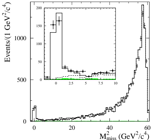
FIG. 7: The M_{\text{miss}}^2 distribution for data (points with error bars) with 2.8 < M_{K^+K^-} < 3.0 \text{ GeV}/c^2 selected with all the criteria described in Sec. III except for the requirement |M_{\text{miss}}^2| < 1 \text{ GeV}^2/c^4 . The solid histogram is a sum of signal and background distributions obtained from MC simulation. The dashed histogram shows the distribution for two-photon events, and the shaded (almost invisible) histogram shows the small contribution of all other background processes. The inset shows an enlarged view of the region -2 < M_{\text{miss}}^2 < 10 \text{ GeV}^2/c^4 . Above 10 \text{ GeV}^2/c^4 the solid and dashed histograms are indistinguishable.
