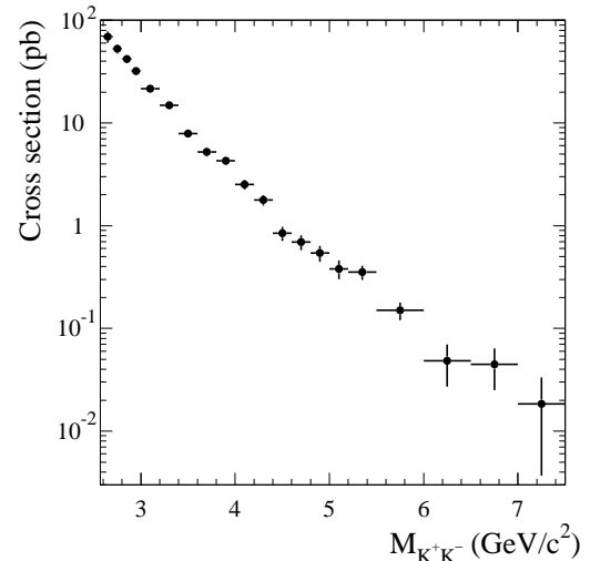
FIG. 10: The e^+e^- \rightarrow K^+K^- cross section measured in this work.
