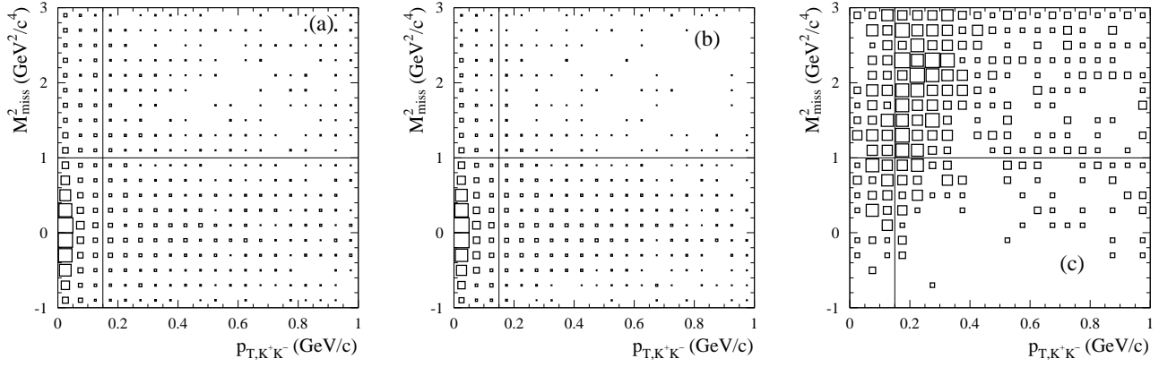
FIG. 5: The distributions of M_{\text{miss}}^2 versus p_{T,K+K^-} for (a) data events, (b) simulated signal events, and (c) simulated ISR background events. Events in the J/\psi and \chi_{c0} mass regions, 3.05 < M_{K+K^-} < 3.15 \text{ GeV}/c^2 and 3.38 < M_{K+K^-} < 3.46 \text{ GeV}/c^2 , are excluded from the distributions; regions near the \chi_{c2} and \psi(2S) are not excluded, since their signal content is quite small. The lines indicate the boundaries of the signal region (bottom left rectangle) and the sideband region (top right rectangle).
