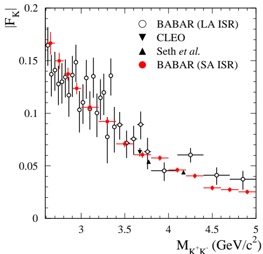
FIG. 11: The charged-kaon electromagnetic form factor measured in this analysis [BABAR (SA ISR)] in comparison with previous measurements: CLEO [8], Seth et al. [9], and BABAR (LA ISR) [3] in the mass region 2.6–5.0 GeV/ c^2 . Only statistical uncertainties are shown.
