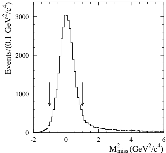
FIG. 2: The M_{\text{miss}}^2 distribution for simulated e^+e^- \rightarrow K^+K^-\gamma events. The arrows indicate |M_{\text{miss}}^2| = 1 \text{ GeV}^2/c^4 .
