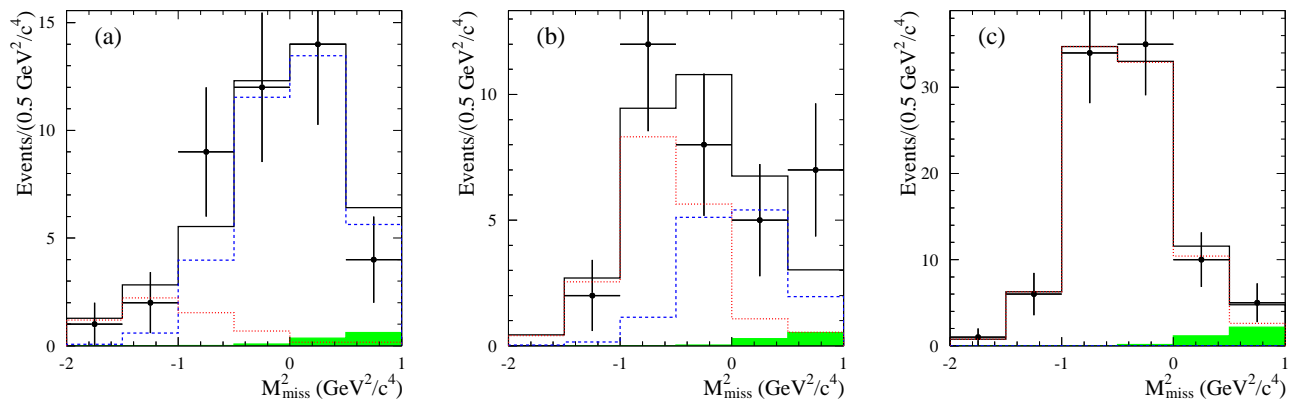
FIG. 4: (Color online) The M_{\text{miss}}^2 distributions for data (points with error bars) in three M_{K+K^-} intervals: (a) 5.5–6.0 \text{GeV}/c^2 , (b) 6.5–7.0 \text{GeV}/c^2 , and (c) 7.5–8.0 \text{GeV}/c^2 . The solid histogram is the result of the fit described in the text. The dashed blue, dotted red, and shaded histograms show the contributions of signal, muon background, and ISR + two-photon background, respectively.
