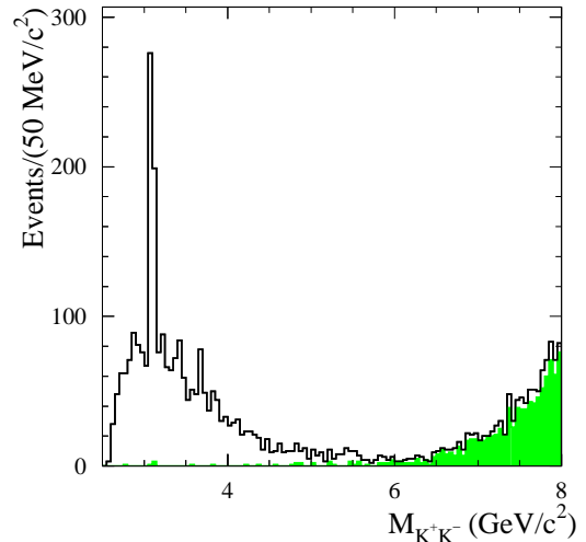
FIG. 3: The K^+K^- mass spectrum for selected K^+K^-\gamma candidates. The peaks near 3.1, 3.4, and 3.7 \text{GeV}/c^2 are from J/\psi , \chi_{c0} , and \psi(2S) decays to K^+K^- , respectively. The shaded histogram shows events with at least one identified muon candidate.
