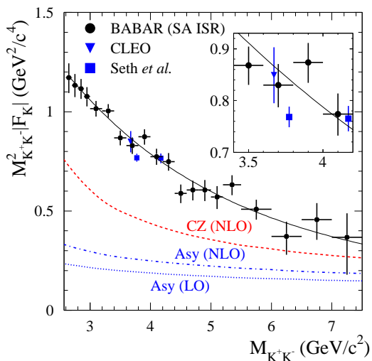
FIG. 12: (Color online) The scaled charged-kaon electromagnetic form factor measured in this analysis [BABAR (SA ISR)] and in other experiments: CLEO [8] and Seth et al. [9]. Our data are approximated by a smooth curve. The dotted blue curve shows the LO pQCD prediction for the form factor obtained with the asymptotic kaon distribution amplitude. The dot-dashed blue and dashed red curves are the NLO pQCD predictions obtained with the asymptotic and Chernyak-Zhitnitsky distribution amplitudes, respectively. The inset shows an enlarged version of the mass region 3.4–4.2 GeV/ c^2 .
