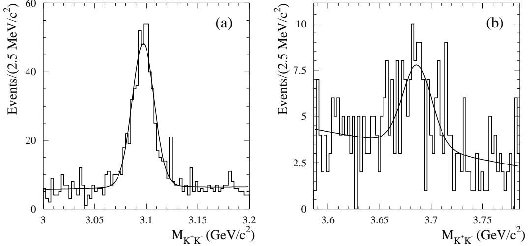
FIG. 13: The K^+K^- mass spectra in the regions near the J/\psi (a) and \psi(2S) (b) resonances. The curves exhibit the results of the fits described in the text.
