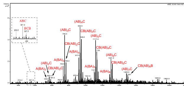
Figure 8. ESI-MS positive ion mass spectrum (100-2000 m/z ) of reaction between PBI and DMA (C) catalyzed by CaLB-Cov. Reaction time: 72 hours.
