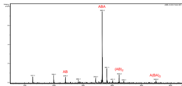
65 Figure 6. Labelled ESI-MS positive ion mass spectrum of polycondensation products of DMI (A) with BDO (B) catalyzed by CaLB-Cov (72 hours).
