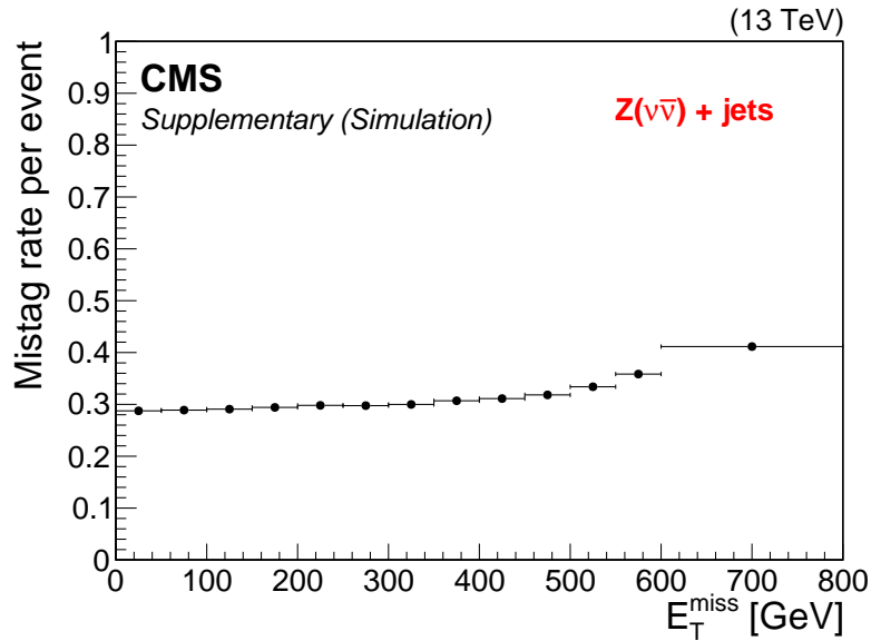
Figure 2: The event mistag rate of the top quark tagger as a function of E_T^{\text{miss}} in the Z \rightarrow \nu\nu simulated sample, with the following event selection requirements applied: N_j \geq 4 for p_T > 30 GeV, |\eta| < 2.4 and N_j \geq 2 for p_T > 50 GeV, |\eta| < 2.4 ; no electrons, muons, or isolated tracks; \Delta\phi(E_T^{\text{miss}}, \text{jets}) matching preselection requirements; and N_b \geq 1 .
