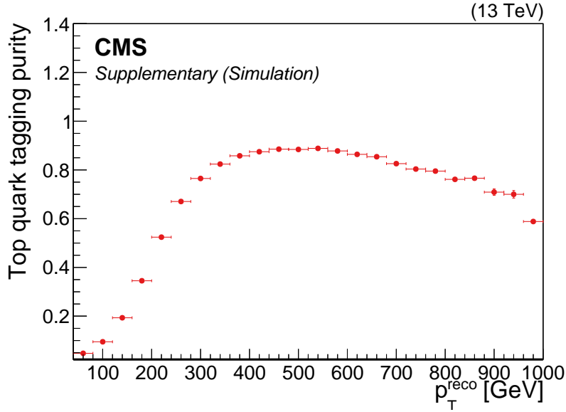
Figure 1: The purity of the top quark tagger as a function of the reconstructed top quark p_T . The purity is defined as the fraction of reconstructed top quarks that are matched to a generator-level hadronically decaying top quark within a cone of \Delta R = 0.4 , and was measured in a sample of simulated one-lepton t\bar{t} events. The following event selection requirements were applied: N_j \geq 4 for p_T > 30 GeV, |\eta| < 2.4 and N_j \geq 2 for p_T > 50 GeV, |\eta| < 2.4 ; N_b \geq 1 ; and E_T^{\text{miss}} > 200 GeV.
