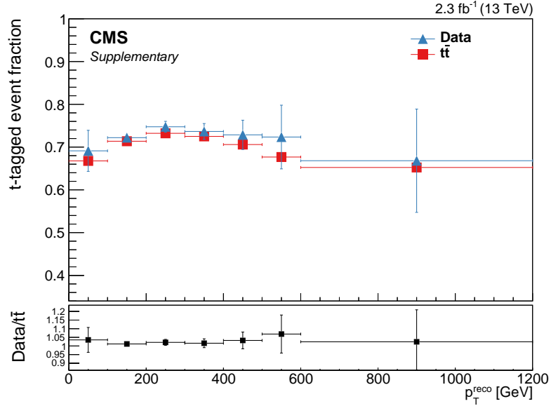
Figure 3: The t -tagged event fraction measured in data and t\bar{t} simulated samples, as a function of the reconstructed top quark candidate p_T . The data are selected from a single muon dataset with the following selection applied: events pass noise filters; N_j \geq 4 for p_T > 30 GeV, |\eta| < 2.4 and N_j \geq 2 for p_T > 50 GeV, |\eta| < 2.4 ; at least one muon with p_T > 45 GeV, |\eta| < 2.1 ; no electrons; muon p_T + E_T^{\text{miss}} > 150 GeV; \Delta\phi(E_T^{\text{miss}}, \text{jets}) matching preselection requirements; N_b \geq 1 ; and E_T^{\text{miss}} > 20 GeV. We also require the presence of at least one candidate from the t -tagger in the event. This candidate can be either: (i) a trijet candidate, composed of three jets with p_T > 30 GeV that are within \Delta R = 1.5 of the candidate four-momentum, (ii) a dijet candidate, composed of two jets that are within \Delta R = 1.5 of the candidate four-momentum, one of which should have a mass between 70 and 110 GeV, or (iii) a monojet candidate, which is simply a single jet with a mass between 110 and 220 GeV. The candidate used to compute the t -tagged event fraction is the candidate whose mass is closest to the top quark mass. The t -tagged event fraction then is defined as the fraction of events for which this top quark candidate satisfies all requirements of the top quark tagging algorithm. The error bar depicts the statistical uncertainty. The ratio of the t -tagged event fraction in data and simulated t\bar{t} is shown in the lower plot, indicating good agreement.
