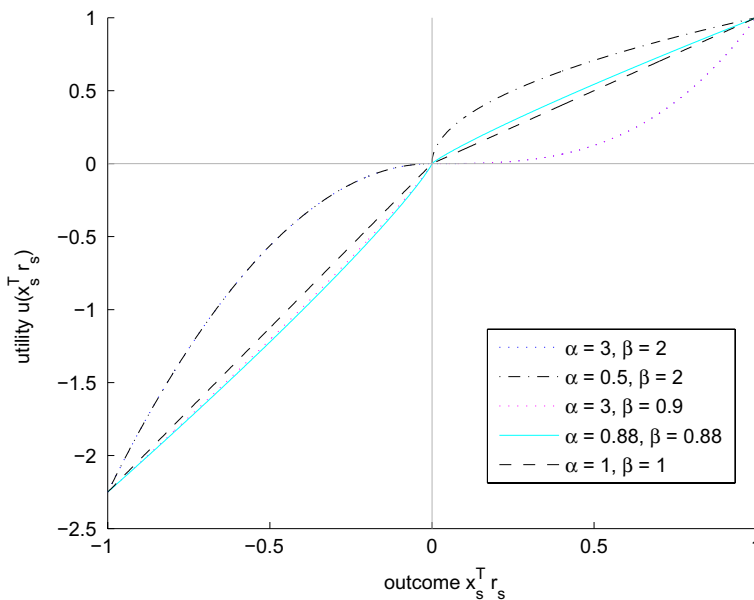
Figure 1. Plots of the utility function given by (19) for \gamma = 2.25 and various \alpha, \beta values. Source: Calculated by the authors.
