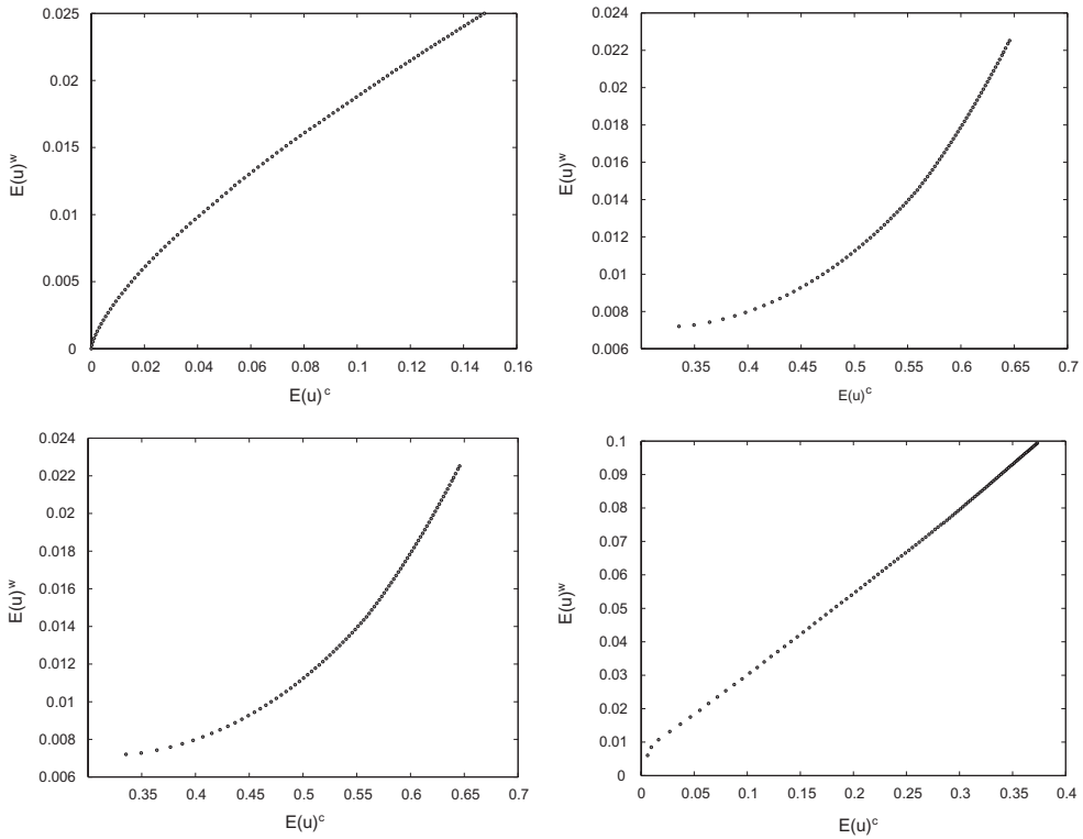
Figure 2. Plot of the non-dominated front found by M.O.E.A./D.-D.E. for each instance of Problem (28) related to investor behaviour. Source: Calculated by the authors.
