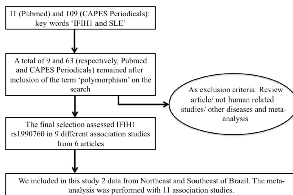
Figure 1. Schematic workflow indicating the criteria for meta-analysis.
