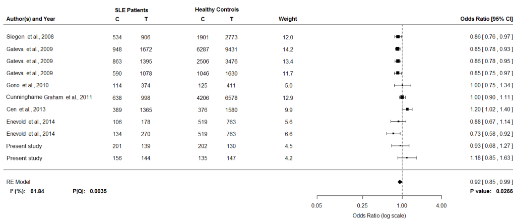
Figure 3. Allele model depicting all studies included in meta-analysis of SNP rs1990760.
