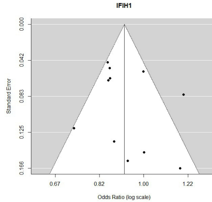
Figure 2. Asymmetry test funnel plot graph for meta-analysis.
