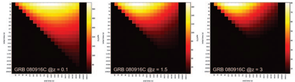
Fig. 3. – TS maps ( z -axis) vs. start ( y -axis) and end time ( x -axis) of the simulation for GRB 080916C placed at three different redshifts.
