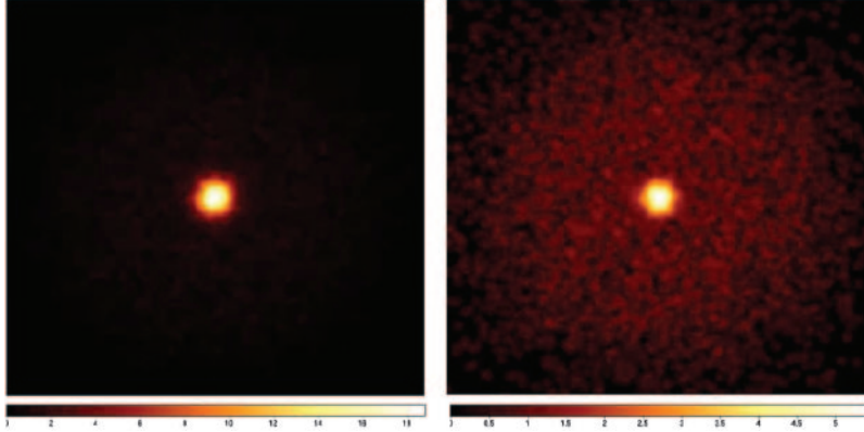
Fig. 1. – Simulations of GRB 130427A with ctools . The camera images are divided into 200 \times 200 bins of 0.02^\circ . The color scale gives the counts/bin after Gaussian smoothing. Left panel: Count map for an observation lasting 10 min starting from 1 ks after the trigger. Right panel: Count map for an observation lasting 0.5 hr starting from 10 ks after the trigger.
