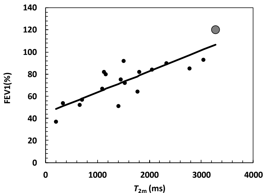
Figure 6. Relation between FEV1 (Forced Expiratory Volume in the first second) and sputum mean relaxation time ( T_{2m} ) referring to CF patients. Black circles represent experimental data, while the solid line is the linear interpolant. Gray large dot indicates healthy subjects.
