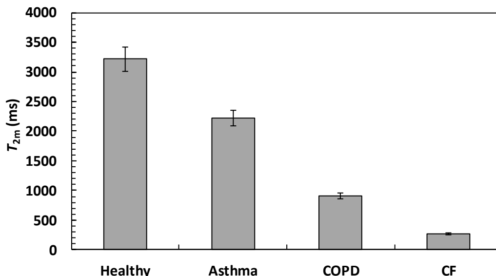
Figure 5. Sputum mean relaxation time ( T_{2m} ) referring to healthy subjects and three patients suffering, respectively, from asthma, COPD (lung bacterial infection), and cystic fibrosis (37 °C). Vertical bars indicate data standard error.
