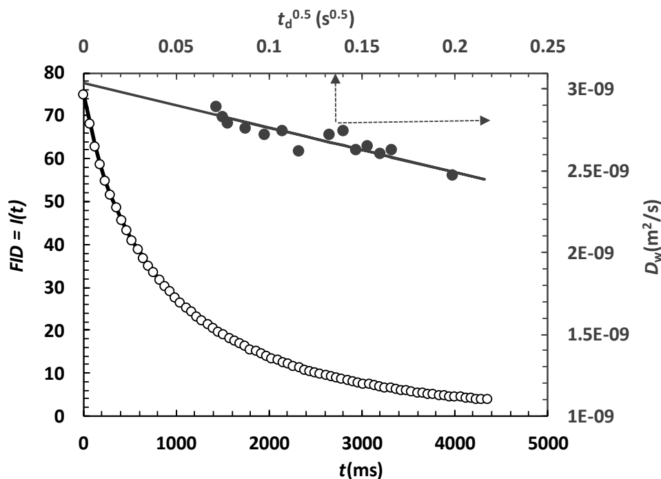
Figure 4. PLLA scaffold (37 °C). a) Left vertical axis (FID) and bottom horizontal axis (time t ): Equation (20) (solid black line) best fit to relaxation data (open circles). b) Right vertical axis (water self-diffusion coefficient D_w ) and top horizontal axis (square root of the diffusion time t_d ): Equation (16) (solid gray line) best fit to experimental data (gray circles). Dashed arrows help to catch the correct vertical and horizontal axis. Adapted from [20].
