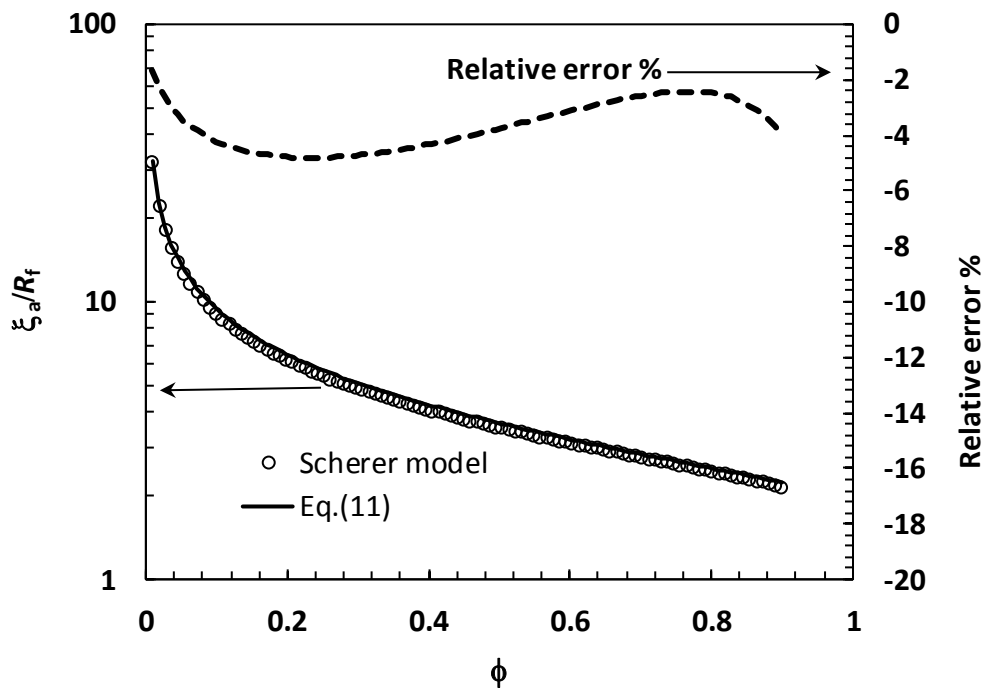
Figure 1. Comparison between Scherer’s model (Equation (6), open circles) and our approximation (Equation (11), solid line, cubic arrangement). The dotted line indicates the relative % error (right vertical axis), \phi is the polymer volume fraction characterizing the network, R_f is the radius of the cylinder able to contain each polymeric chain in its linear configuration, while \xi_a is the average mesh size.
