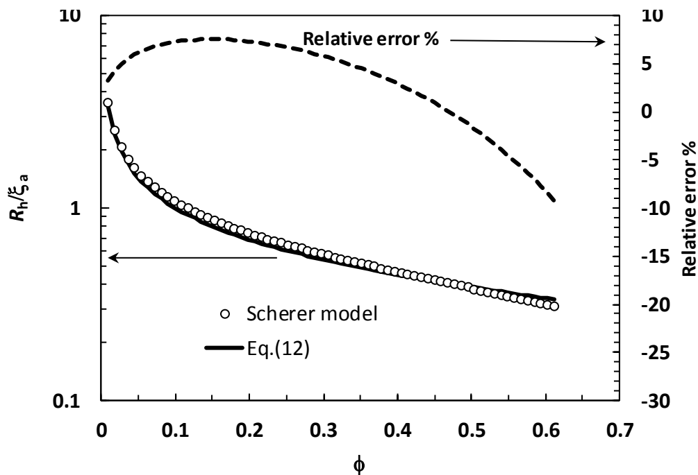
Figure 2. Comparison between Scherer’s model (Equation (6), open circles) and our approximation (Equation (12), solid line, cubic arrangement). The dotted line indicates the relative % error (right vertical axis), \phi is the polymer volume fraction characterizing the network, R_h is the hydraulic radius, and \xi_a is the average mesh size.
