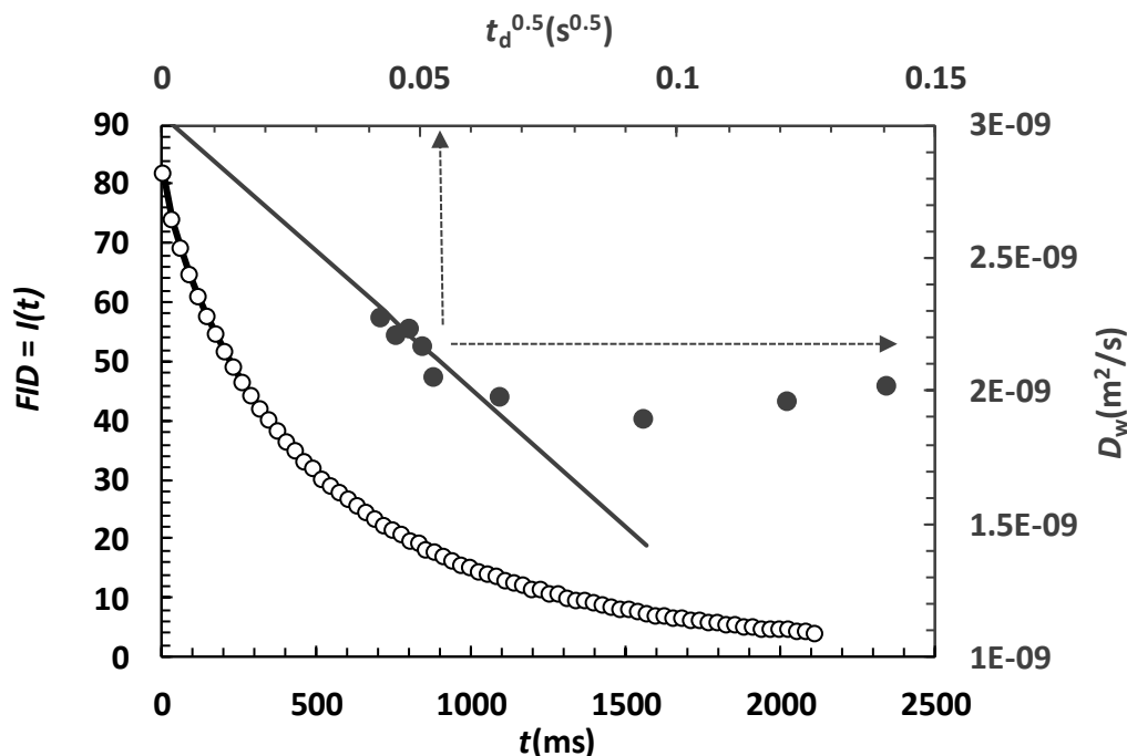
Figure 3. Porous hydrogel composed of acrylic acid and bacterial cellulose (37 °C). a) Left vertical axis (FID) and bottom horizontal axis (time t ): Equation (20) (solid black line) best fit to relaxation data (open circles). b) Right vertical axis (water self-diffusion coefficient D_w ) and top horizontal axis (square root of the diffusion time t_d ): Equation (16) (solid gray line) best fit to experimental data (gray circles). Dashed arrows help to catch the correct vertical and horizontal axis. Adapted from [37].
