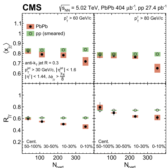
Fig. 7. The \langle x_{jy} \rangle (top) and R_{jy} (bottom) as a function of \langle N_{\text{part}} \rangle for p_T^{\gamma} > 60 GeV/c (left) and p_T^{\gamma} > 80 GeV/c (right). The PbPb results (full markers) are compared to pp results (open markers) smeared by the relative jet energy resolution corresponding to each centrality interval. The vertical lines (bands) through the points represent statistical (systematic) uncertainties.
