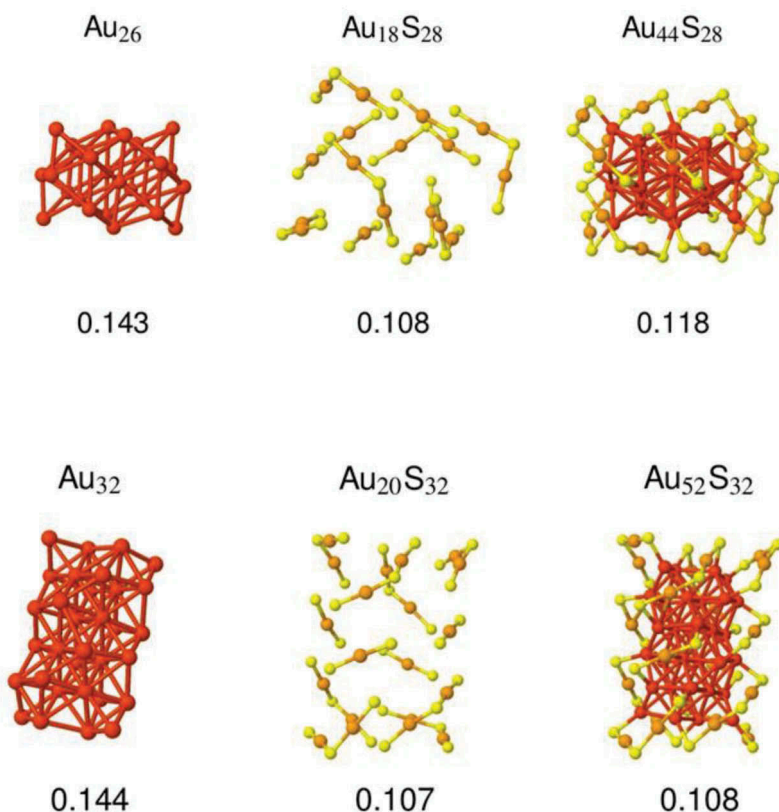
Figure 6. Structures and HCM values for the cluster core, ligand shell (Au–S interface), and protected cluster. Top panel: \text{Au}_{44}(\text{SR})_{28} ; bottom panel: \text{Au}_{52}(\text{SR})_{32} . Core Au atoms are in red, shell Au atoms are in dark yellow, and S are in light yellow. This figure is adapted from the original one reported in Ref. [77].
