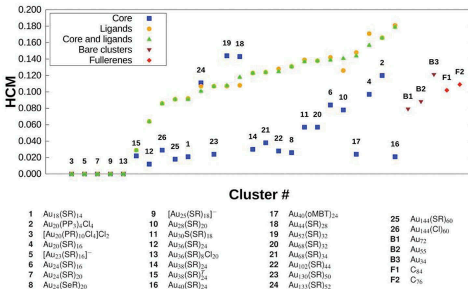
Figure 7. HCM index of chirality for ligand-protected gold clusters. The numbers in black above the blue squares denote the cluster number according to the list shown in the bottom panel. This figure is adapted from the original one reported in Ref. [77].
