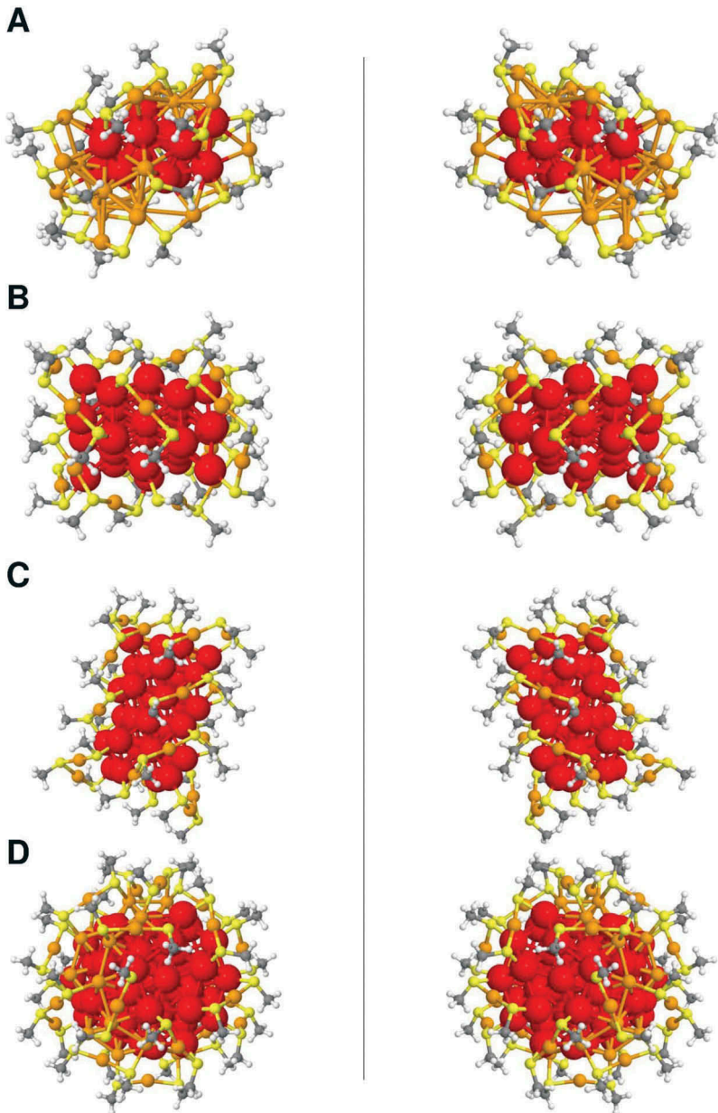
Figure 3. Structures of chiral thiolate-protected gold clusters. (a) \text{Au}_{38}(\text{SCH}_3)_{24} , (b) \text{Au}_{44}(\text{SCH}_3)_{28} , (c) \text{Au}_{52}(\text{SCH}_3)_{32} , and (d) \text{Au}_{102}(\text{SCH}_3)_{44} .
