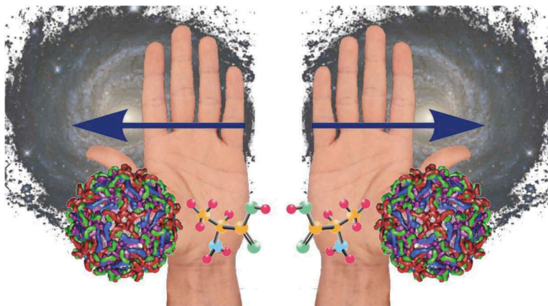
Figure 1. Different chiral systems that exist in our universe.
