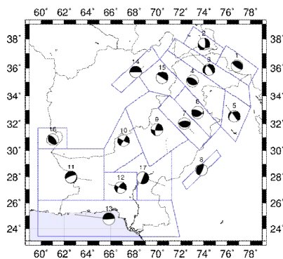
Fig. 5. Boundaries of the seismogenic zones, and the focal mechanism associated with the sources belonging to each seismogenic zone.
