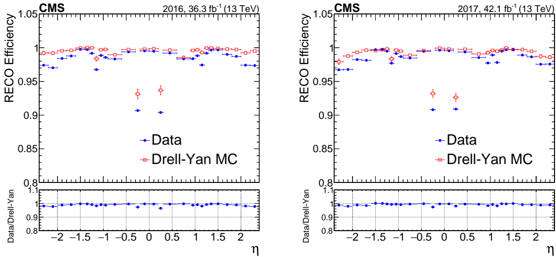
Figure 7. Stalone muon reconstruction efficiency as a function of muon \eta for the (left) 2016 and (right) 2017 data sets. The blue points represent the data, while the red empty squares represent the simulation.
