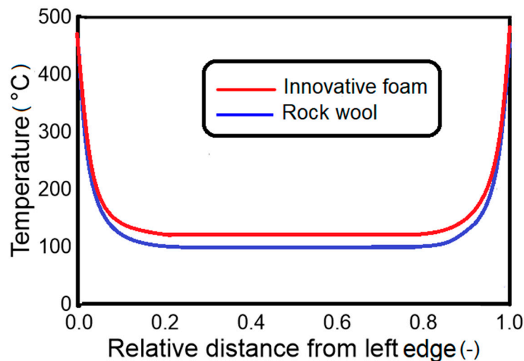
Figure 9. Transversal temperature profile at the final stage of the fire test (60 min) along the line passing through measuring point 5 (see black line in Figure 1b): comparison between foam and rock-wool model.
