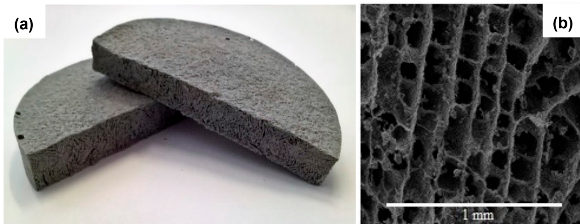
Figure 3. (a) Fiberglass foam; (b) fiberglass foam microstructure.
