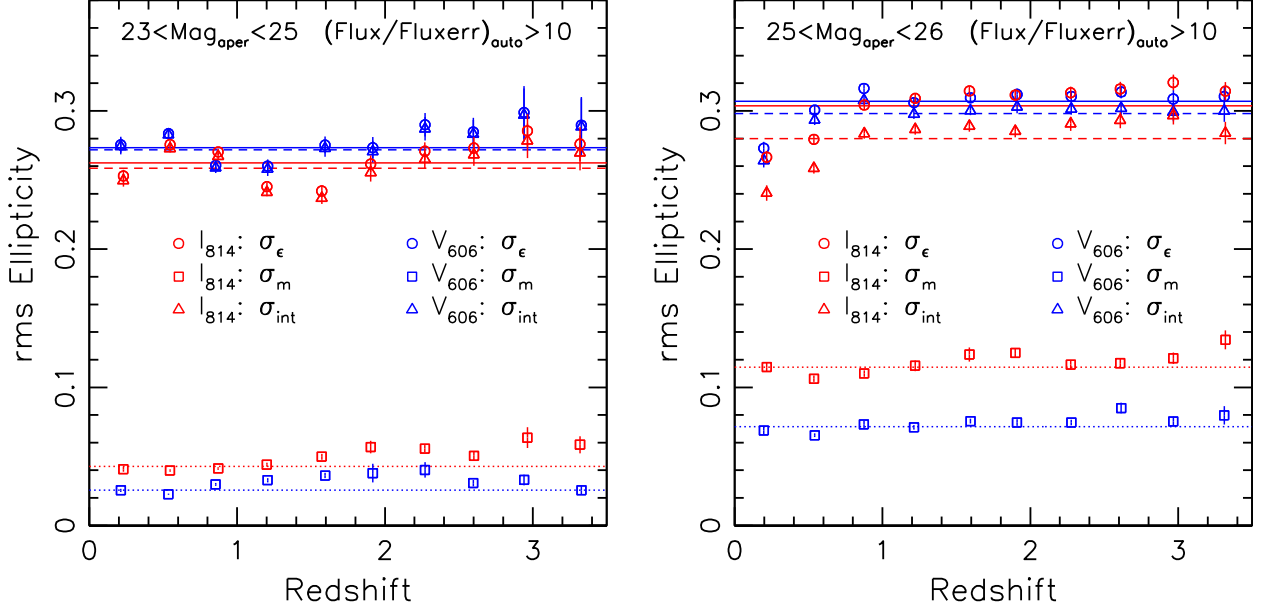
Figure A4. Galaxy ellipticity dispersion per ellipticity component as a function of photometric redshift for bright 23 < \text{mag} < 25 galaxies ( left ), and faint 25 < \text{mag} < 26 galaxies ( right ). The horizontal lines show the weighted averages. See the caption of Fig. A1 for further details.
