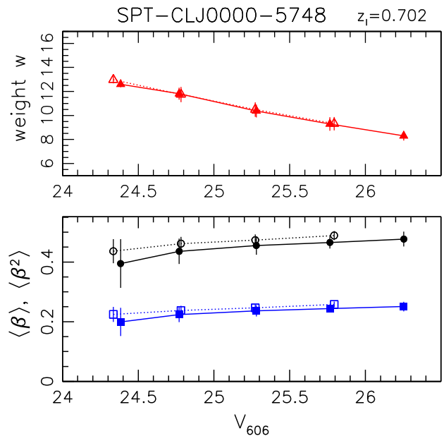
Figure 8. Analysis of SPT-CL J0000–5748 as a function of V_{606} magnitude, where the solid (open) symbols correspond to the ACS-only (ACS+FOR2) analysis. Top: Mean weak lensing shape weight w with error-bars indicating the dispersion from all selected galaxies in the magnitude bin. Bottom: \langle \beta \rangle (circles) and \langle \beta^2 \rangle (squares) with error-bars showing the dispersion of their estimates computed from all CANDELS sub-patches (see Section 6.6), thus indicating the expected line-of-sight variations for the field sizes of our cluster observations.
