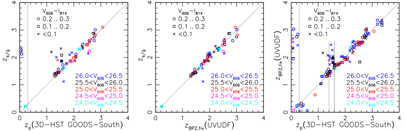
Figure 6. Comparison of redshift estimates in the HUDF including the peak photometric redshift from EAZY z_p estimated by the 3D-HST team in the GOODS-South field, the BPZ photometric redshift from the UVUDF project z_{\text{BPZ,fix}} (with small bias corrections applied, see text), and a combined sample of spectroscopic and grism redshifts z_{\text{s/g}} . We regard the latter as a true but incomplete reference sample, which reveals the presence of significant outliers for the z_p but not the z_{\text{BPZ,fix}} photo- z s. We therefore use the z_{\text{BPZ,fix}} photo- z s, which do not suffer from incompleteness at the relevant depth, to derive a statistical correction for the z_p photo- z s. The symbols split the galaxies according to V_{606} - I_{814} colour and the different colours indicate different magnitude bins (based on the 3D-HST photometry). Galaxies are only included if they pass our weak lensing selection and if they are located within the area covered by the WFC3 UVIS and IR observations. In the right-hand panel the vertical lines indicate the z_p ranges of our statistical correction for the redshift distribution.
