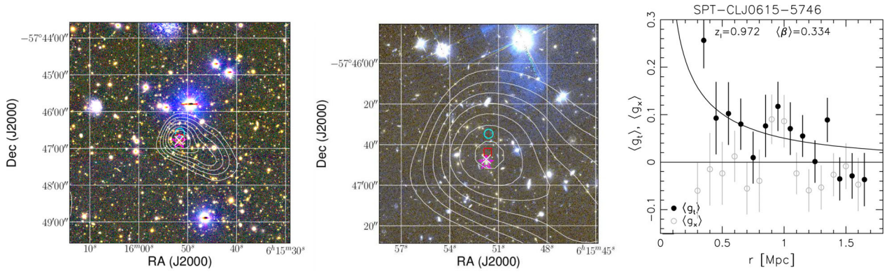
Figure G6. Weak lensing results for SPT-CLJ0615–5746. See the descriptions in the captions of Figs 14 and 16 for details.
