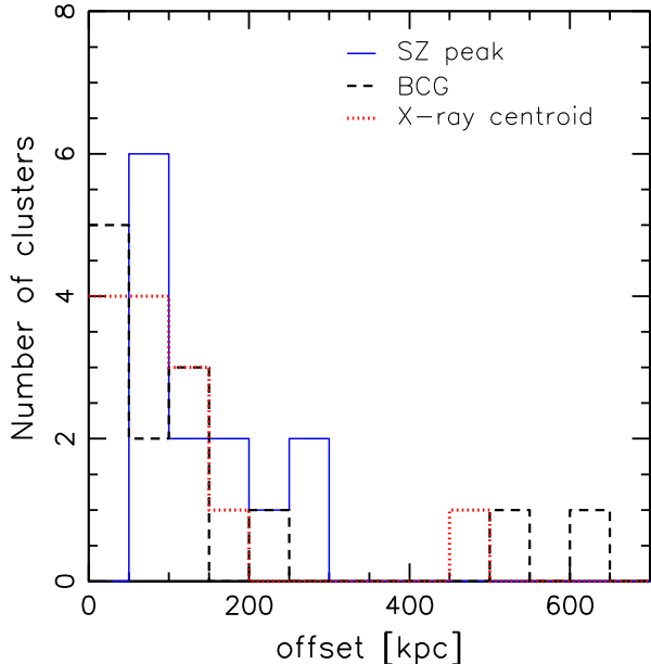
Figure 15. Histograms of spatial offsets between the peak in the mass reconstruction signal-to-noise map and the indicated centres.
