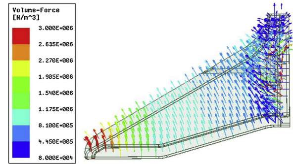
Fig. 6. Force density arising from a toroidal field of 1.43 T and a current of 4 kA flowing from the tile tip to the rail.
