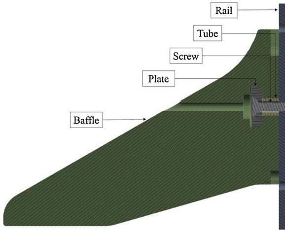
Fig. 4. CAD model assembly.
