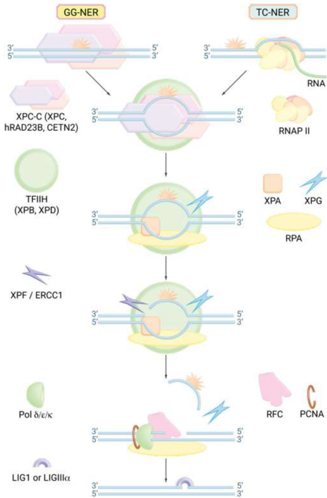
Fig. 10. Schematic representation of the human NER pathway.
