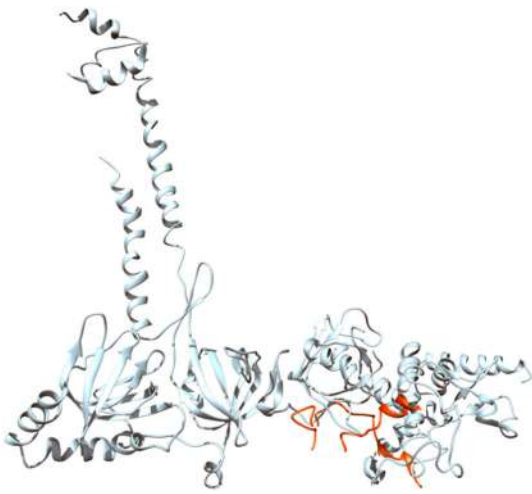
Fig. 27. Overall view of the COOH-terminal domain of BRCA2 (light blue) bound to DSS1 (orange) (PDB: 1MIU (H. Yang et al., 2002)).
