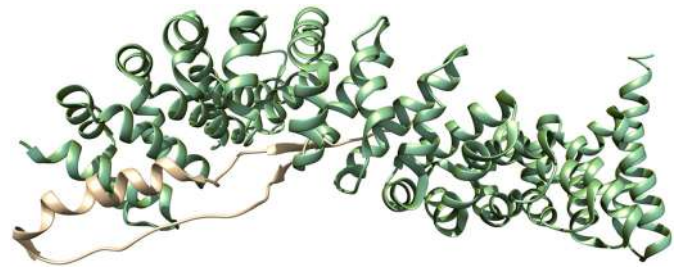
Fig. 47. Crystal structure of the E-cadherin cytoplasmic domain (light tan) complexed with the so-called armadillo repeat region of \beta -catenin (olive drab) (PDB: 1I7X (Huber & Weis, 2001)).
