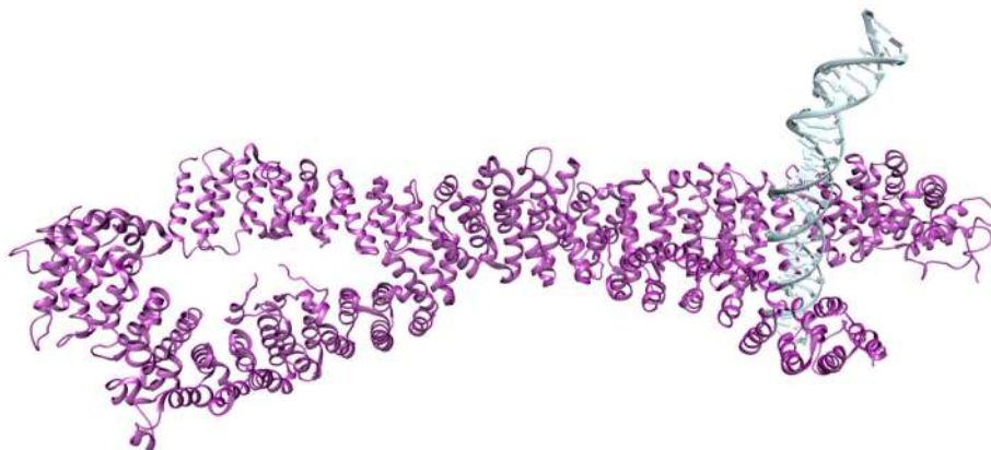
Fig. 17. Crystal structure of the N-terminal domain of RIF1 (magenta) binding to DNA (light blue) and suppressing its end resection, promoting repair by NHEJ (PDB: 5NW5 (Matarrocci et al., 2017)).
