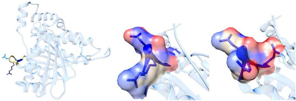
Fig. 43. (Left) The three RAD51 residues D149 (dodger blue), R150 (dark slate blue), and G151 (navy blue) belonging to the Schellman loop (kaki) found mutated in BC. Zoomed views of the variation in the shape, size, and local surface electrostatic properties obtained by replacing the wild type RAD51 D149, R150, and G151 residues (middle) with the three mutants N149, Q150, and D151 (right). Blue regions indicated electropositive character of the surface, while red regions indicate electronegative surface characteristics. For simplicity, all three residues have been changed in the right panel; however, each missense mutation was singularly detected in the clinical samples (PDB: 5JZC (Short et al., 2016)).
