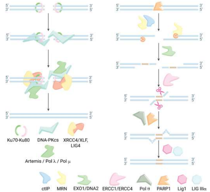
Fig. 18. The pathways of cNHEJ (left) and aNHEJ (right).
