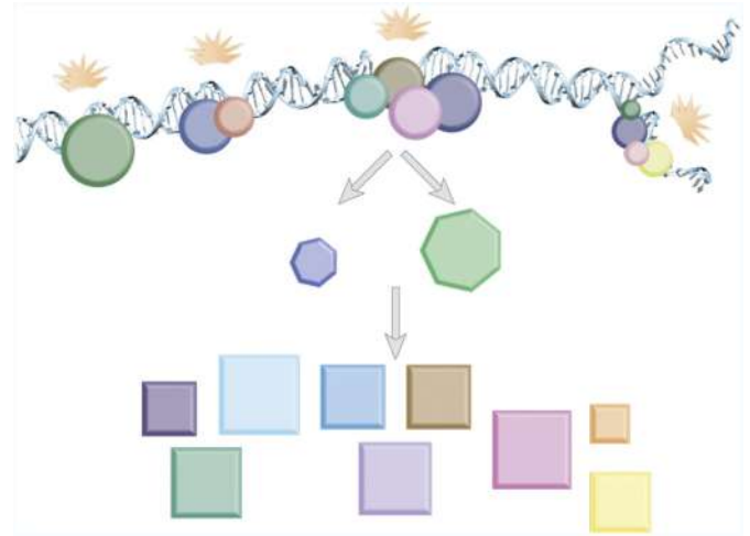
Fig. 5. Schematic representation of cellular response to DNA damage. Multiple sensor proteins (colored circles) are initially involved in recognizing the different nucleic acid lesion (light orange pointed symbols). Other transducer proteins (colored hexagons) then amplify and diversify the DNA-damage signal, and a plethora of downstream effectors (colored squares) regulate various aspects of the cellular function, including replisome stability, transcription, cell cycle, energy and autophagy, chromatin remodeling, repair, RNA processing, apoptosis and senescence.
