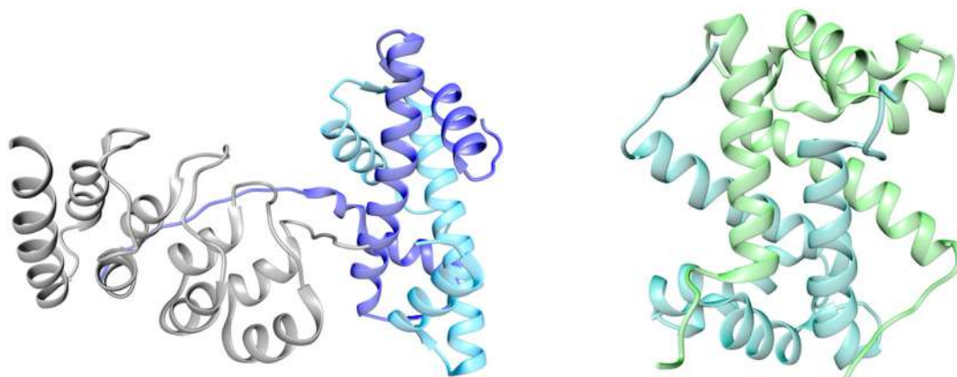
Fig. 33. (Left) Crystal structure of the human TONSL (gray) binding to a histone H3 (sky blue)-H4 (medium blue) tetramer (PDB: 5JA4 (Saredi et al., 2016)). (Right) NMR-derived structure of the SA100-A11 homodimer in solution (PDB: 2LUC (Hung, Chang, & Yu, 2012)).
