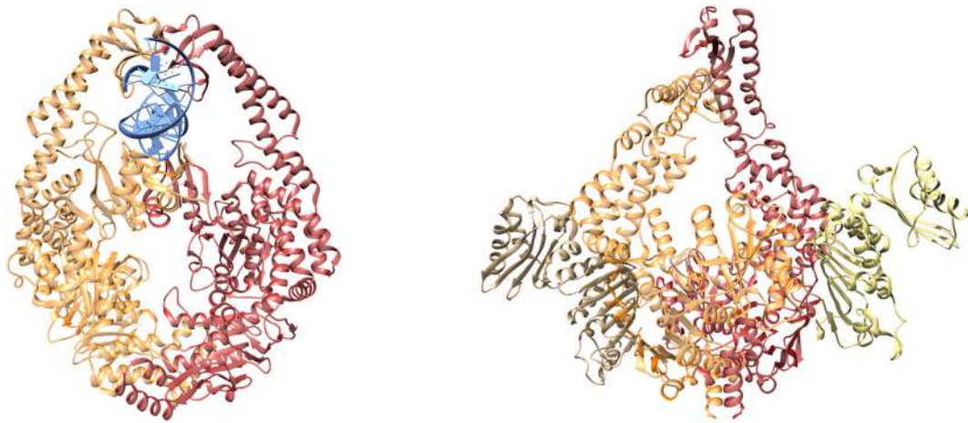
Fig. 8. (Left) Crystal structure of the mutS \alpha sliding clamp (orange and firebrick ribbons) bound to DNA (light blue) upon mismatch identification during MMR (PDB: 3ZLJ (Groothuizen et al., 2013)). (Right) Crystal structure of the mutS \alpha /mutL \alpha tetrameric sliding clamp (mutS \alpha : orange and firebrick ribbons; mutL \alpha , tan and khaki ribbons; PDB: 5AKB (Groothuizen et al., 2015)).
