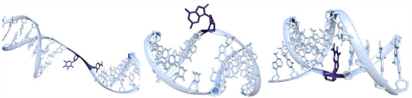
Fig. 2. Models of a DNA SSB (left), a DNA carrying an 8-oxoG lesion (middle), and a DNA with a cyPu adduct (right). Colors as in Fig. 1.
