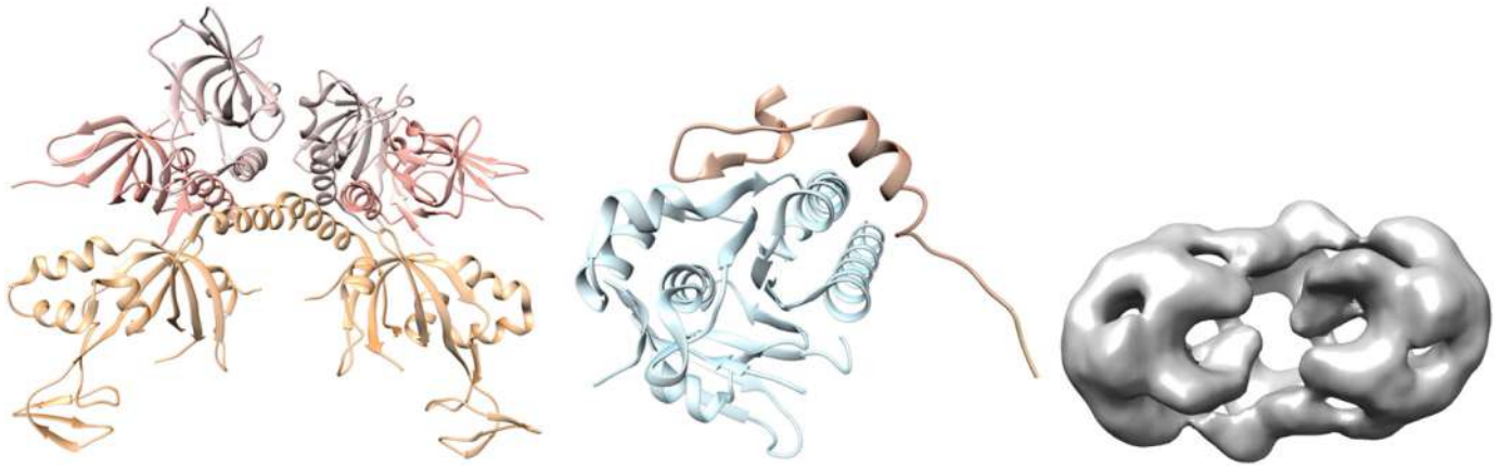
Fig. 26. (Left) The structure of the RPA trimerization core comprising the C-terminal DNA-binding domain of subunit RPA70 (DBD-C), the central DNA-binding domain of subunit RPA32 (DBD-D) and the entire RPA14 subunit (PDB: 1L10 (Bochkareva et al., 2002)). (Middle) The structure of a complex between an evolutionarily conserved sequence in BRCA2 (the BRC repeat, sienna) and the core domain of RAD51 (light blue) (PDB: 1NOW (Pellegrini et al., 2002)). (Right) Surface view of the 3D reconstruction of the BRCA2 dimer as obtained from EM (Electron Microscopy Data Bank (EMD): 2779 (Shahid et al., 2014)).
