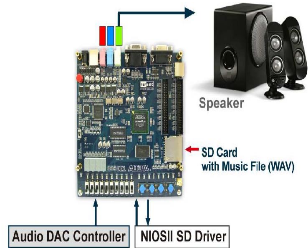
Fig. 5. The setup for the implemented test.
