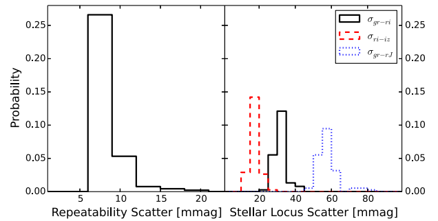
Figure 1. Distribution of single-epoch photometric repeatability scatter (left-hand panel) for multiple measurements of the same stars in our ensemble of 74 clusters. The bands griz have a median scatter of 7.6, 7.6, 7.7 and 8.3 mmag, respectively. The distribution of orthogonal scatter about the stellar locus is shown on the right for three colour–colour spaces. The scatter distributions for these three spaces have a median scatter of 17, 32 and 57 mmag.
