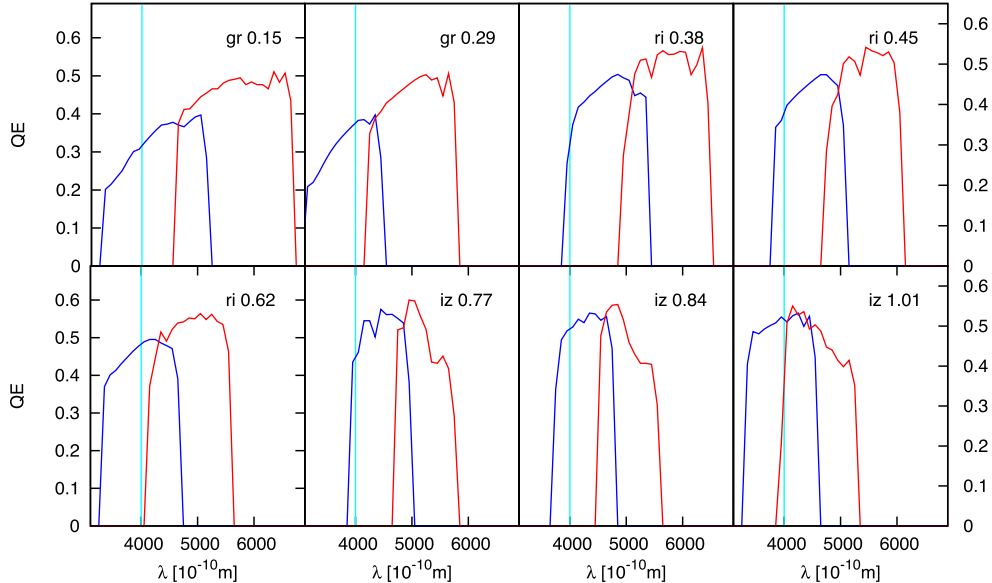
Figure 5. Plots of the average relative throughput or quantum efficiency (QE) in the rest frame of the blue and red bands we use within the eight different redshift bins defined in Table 2. Redshifts and observed band combinations are noted in each panel, and 4000 Å is marked in cyan. By adopting different band combinations as a function of redshift, we are able to probe similar portions of the rest-frame SED over the full redshift range.
