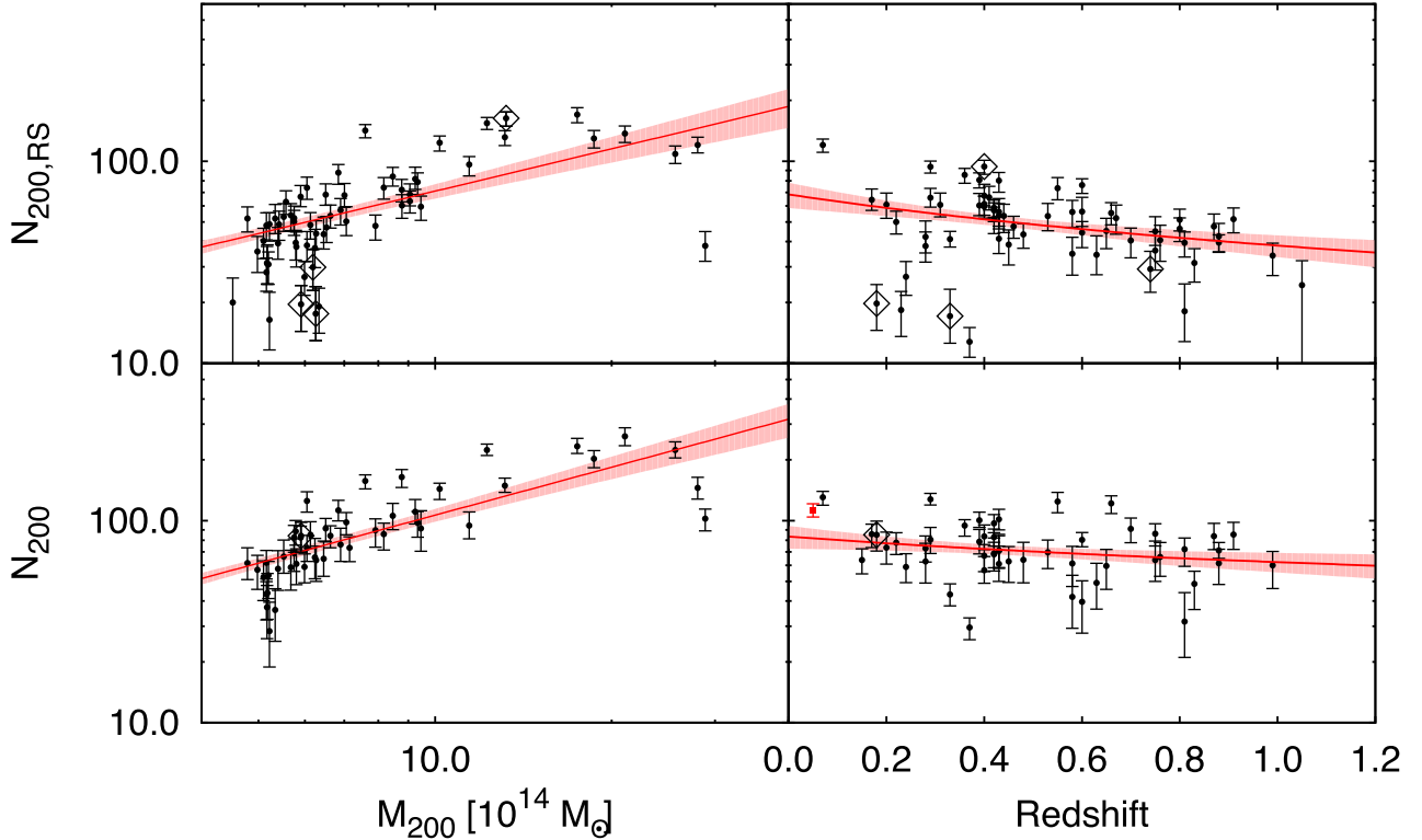
Figure 14. The HON from measurements of N_{200} from the galaxy radial profiles is plotted versus mass (left-hand panels), and the HON normalized to a mass of 6 \times 10^{14} M_{\odot} is plotted versus redshift (right-hand panels). In both cases, the full (RS) population appears on bottom (top panel), and both populations have N_g \propto M^B , where B < 1 (see Table 4). We find no clear evidence of a redshift trend in the full population, but the RS population shows a 2.5\sigma trend for falling HON with redshift. The 1\sigma region (equation 14) for each fit is plotted in red. The clusters near the LMC ( \delta < -63^\circ ) are more contaminated by stars and are marked with black open diamonds.
