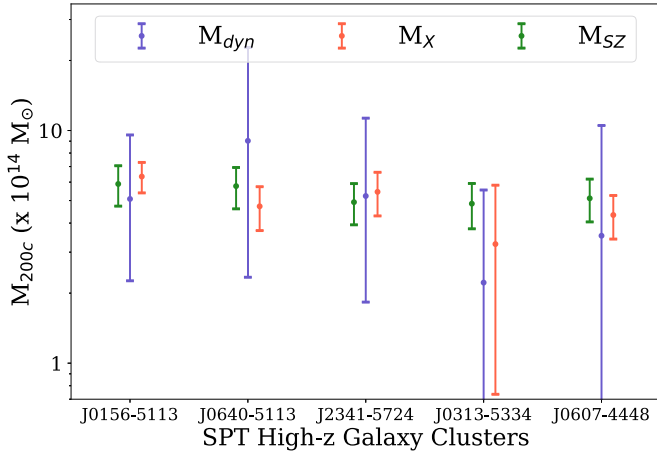
Figure 8. M_{200c} comparisons for the SPT High- z cluster sample—dynamical (purple), X-ray (orange), and SZ (green). The M_{200c,dyn} calculated in this paper are not inconsistent with other published masses for these galaxy clusters (see Table 5 for details).
