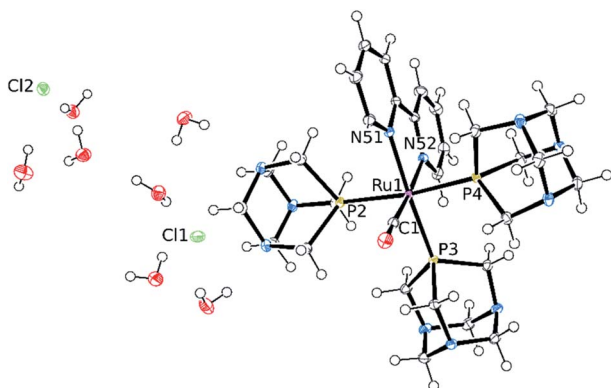
Fig. 4 X-ray molecular structure (50% probability ellipsoids) of mer -[Ru(bpy)(CO)(PTA) 3 ](Cl) 2 ·7H 2 O ( 12 ·7H 2 O) obtained by recrystallization of the raw product from water/acetone. Coordination distances (Å): Ru1–C1 = 1.8746(14), Ru1–N51 = 2.119(1), Ru1–N52 = 2.139(1), Ru1–P2 = 2.3650(4), Ru1–P3 = 2.3391(4), Ru1–P4 = 2.3631(4).
