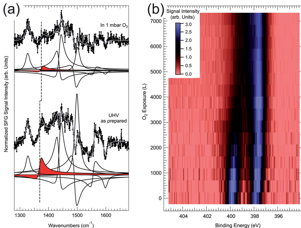
Fig. 7 (a) IR-Vis SFG spectra of the pristine 2H-TTP/Pd(100) monolayer in UHV (bottom) and in 1 mbar \text{O}_2 at room temperature (top). (b) NAP-XPS map showing the evolution of the N 1s core level upon exposure of the 2H-TTP/Pd(100) monolayer to oxygen at room temperature (the signal intensity is mapped in arbitrary units following the colour scale represented in the inset). 49
