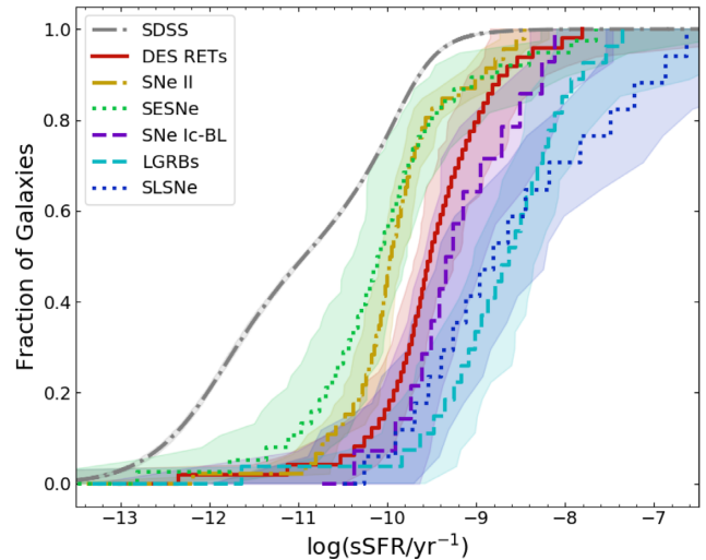
Figure 10. Cumulative distributions of the sSFR of RET hosts, compared to CCSNe and the low- z DSS sample. Uncertainties have been estimated via a bootstrap Monte Carlo technique and include limits.
