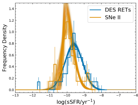
Figure B3. Results of the MCMC fits to the PDFs of sSFR for DES RETs and SNe II, accounting for uncertainties in each bin.
