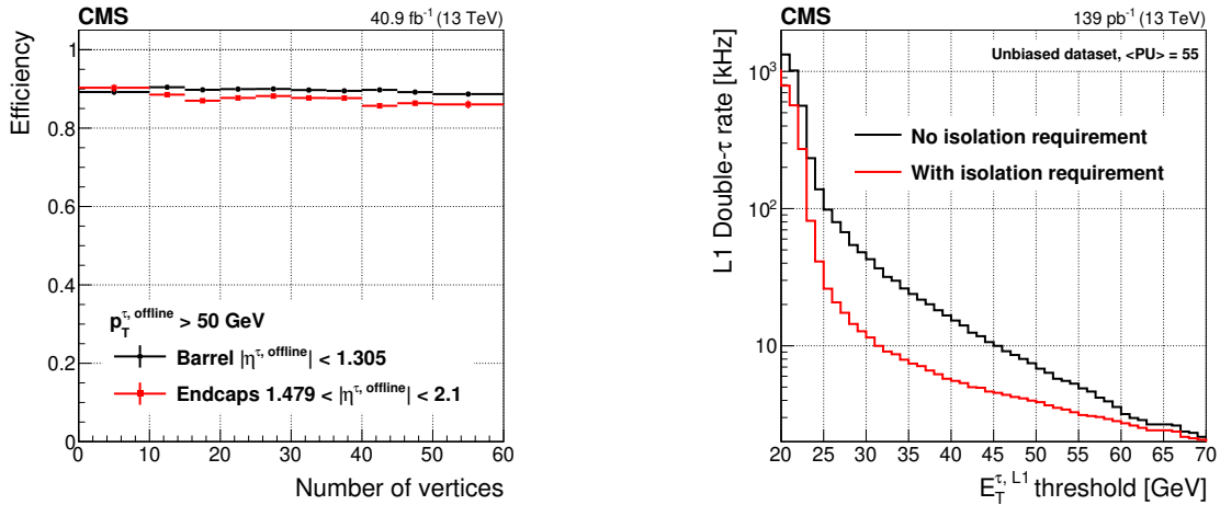
Figure 22. The integrated Level-1 selection efficiency for the isolated \tau trigger with E_T \geq 30 \text{ GeV} , matched to an offline reconstructed and identified \tau lepton with p_T > 50 \text{ GeV} , as a function of the number of offline reconstructed vertices (left). The Level-1 double- \tau trigger rate, as a function of the E_T threshold, for \tau candidates with and without an isolation requirement applied (right). The rate is measured requiring two \tau candidates with E_T larger than the bin value, in a unbiased data set with an average pileup of 55.
