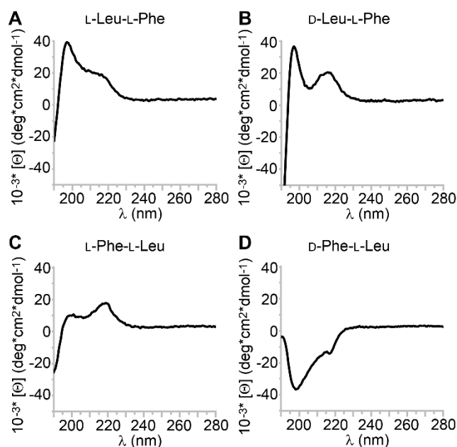
Figure 5. Circular dichroism spectra of the four dipeptides in solution (1 mM).
