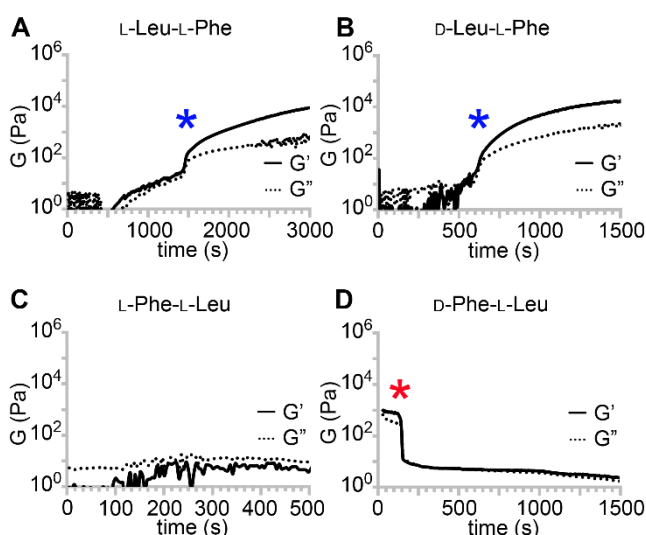
Figure 1. Oscillatory rheology time sweeps for the four dipeptides at 40 mM. Blue stars mark sol-to-gel transitions for the two gelators L-Leu-L-Phe and D-Leu-L-Phe; the red star in (D) marks gel-to-sol transition for the metastable gel formed by D-Phe-L-Leu.
