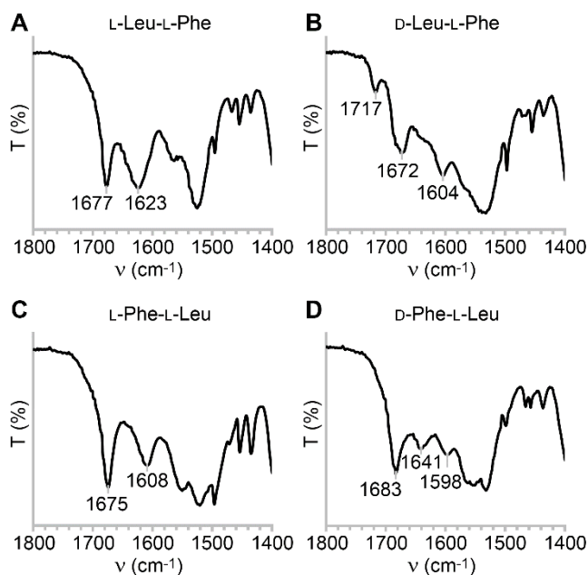
Figure 6. Amide region of the ATR-IR spectra of the four dipeptides in the gel (A,B,D) or precipitate (C) form.
