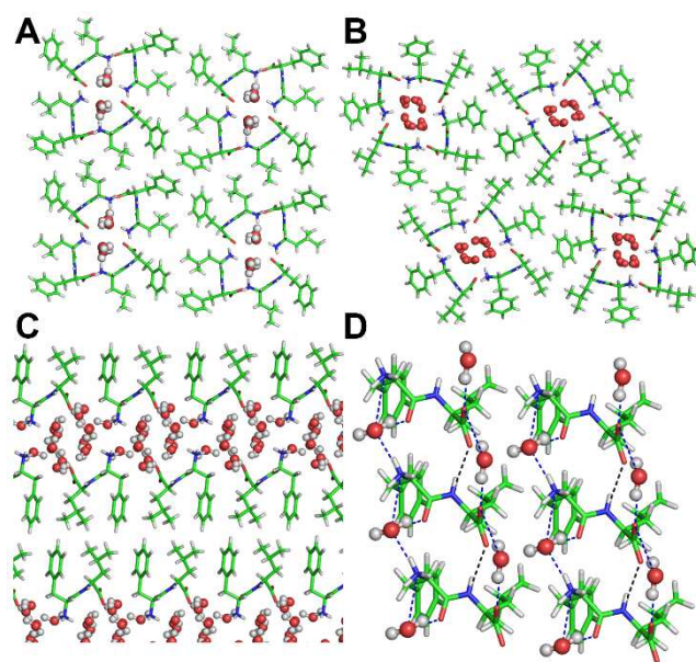
Figure 4. Single-crystal XRD structures of (A) L-Leu-L-Phe, 36 (B) L-Phe-L-Leu, 36 and (C-D) D-Leu-L-Phe (CCDC 2012848), highlighting the alternation of hydrophobic and hydrophilic layers (C) and the hydrogen bonding pattern (D, hydrogen bonding involving only peptide molecules as black dashes, hydrogen bonding involving both peptide and water molecules in blue dashes).
