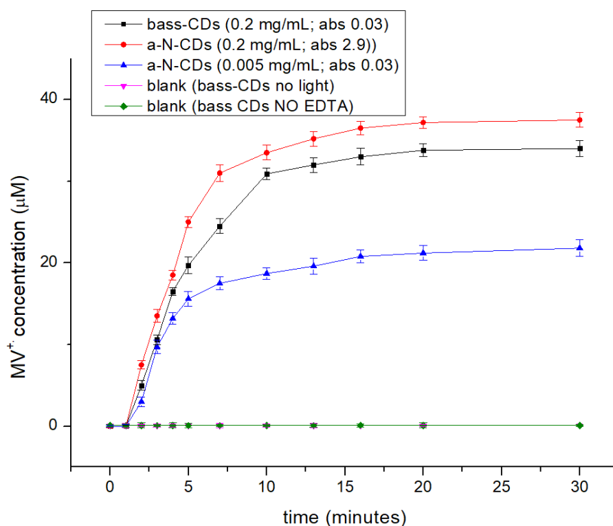
Figure 7. Reaction kinetics of the formation of methyl viologen radical ( \text{MV}^{\cdot+} ) using bass-CDs (black datapoints) and a-N-CDs (red and blue datapoints). Blank tests in absence of light (pink datapoints) and of EDTA (green datapoints).
