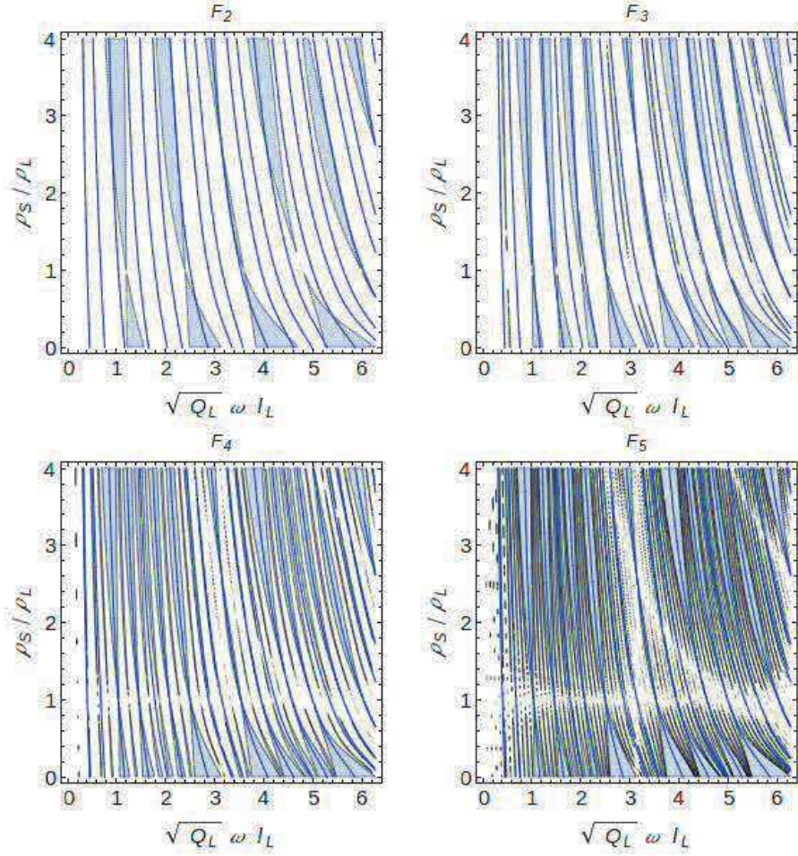
Figure 12: Sector plots of |\text{tr } \mathbf{T}_i| ( i = 2, \dots, 5 ) for SMSs evaluated assuming l_S = l_L/\sigma_g and \rho_S = \rho_L/2 . The band-gap regions ( |\text{tr } \mathbf{T}_i| \geq 2 ) are highlighted in light blue. The thin blue lines denote the local maxima of |H(\omega)| .
