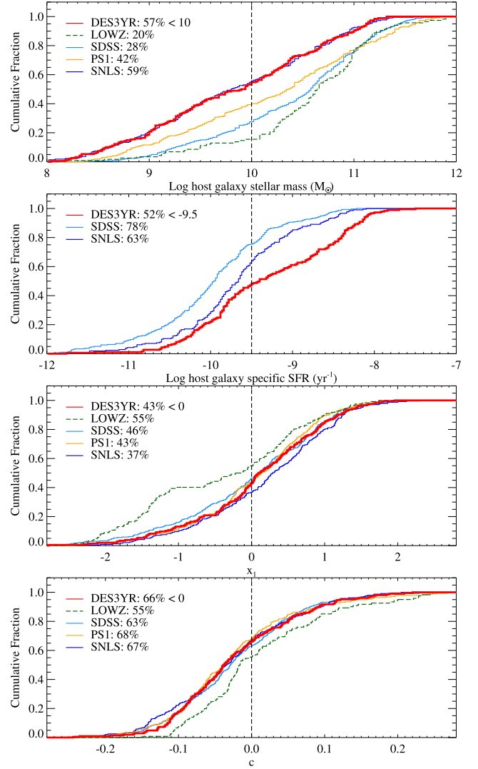
Figure 3. Cumulative distributions of M_{\text{stellar}} , sSFR, x_1 , and c for the DES-SN sample (shown in red) compared to literature data sets (SDSS, light-blue; SNLS, dark blue; PS1, yellow; low-z, green). The fraction of SNe Ia with \log M_{\text{stellar}}/M_{\odot} < 10 , \text{sSFR} < -9.5 , x_1 < 0 , and c < 0 is also shown.
