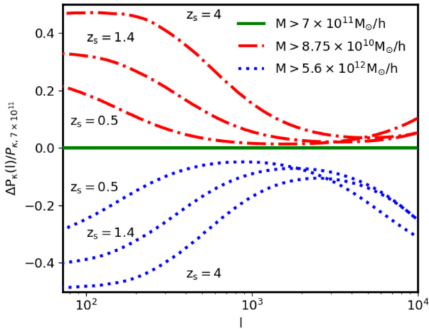
Figure 5. Relative difference of the convergence power spectra, computed using the halo model at three different fixed source redshifts, using different minimum halo mass threshold in the integrals. Left-hand panel shows the relative difference with respect to the prediction of the mass resolution of the reference run of the 1- and 2-halo terms summing the contributions from equation (15) of the expressions in equations (18) and (19). Right-hand panel displays the relative difference of the total contributions where the 2-halo term has been normalized by equation (20).
