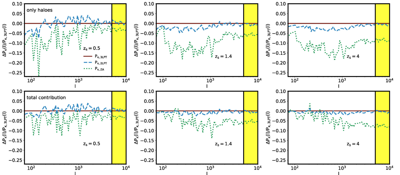
Figure 10. Relative convergence power spectra between maps constructed using PINOCCHIO 2LPT (dashed blue) and ZA (dotted green) with respect to 3LPT. From left to right, we show the cases for the three considered source redshifts: z_s = 0.5 , 1.4, and 4, respectively. Top and bottom panels show the cases in which the maps are constructed using only haloes or haloes plus diffuse matter.
