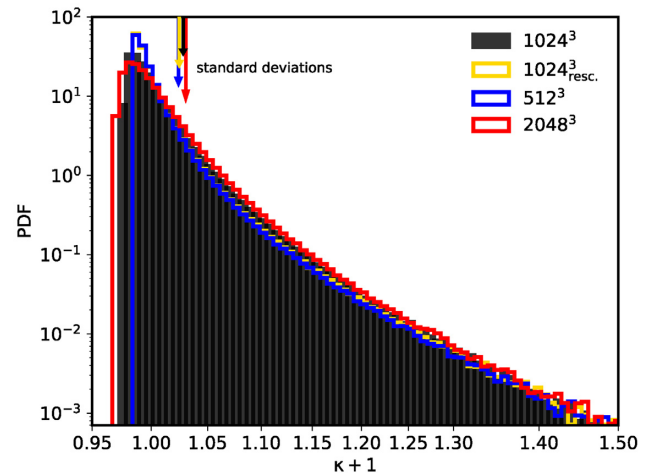
Figure B2. Probability distribution function per pixel of the convergence maps presented in Fig. B1. The arrows mark the standard deviation of the distributions, we recall the reader that by construction the maps have average equal to zero (Hilbert et al. 2020).
