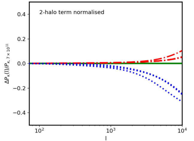
Figure 5. Relative difference of the convergence power spectra, computed using the halo model at three different fixed source redshifts, using different minimum halo mass threshold in the integrals. Left-hand panel shows the relative difference with respect to the prediction of the mass resolution of the reference run of the 1- and 2-halo terms summing the contributions from equation (15) of the expressions in equations (18) and (19). Right-hand panel displays the relative difference of the total contributions where the 2-halo term has been normalized by equation (20).
