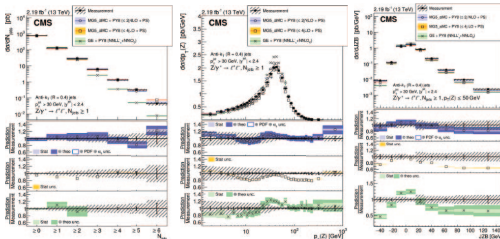
Fig. 2. – Measured cross section for Z + jets as a function of the N_{jets} (left), the p_T of the Z boson (center) and the jet-Z boson imbalance JZB = |\sum_{jets} \vec{p}_T(j_i)| - |\vec{p}_T^Z| (right).
