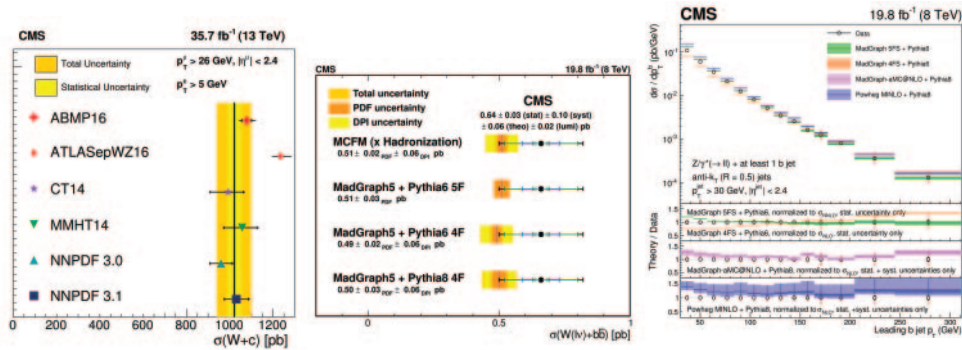
Fig. 4. – Measured cross section for W+c (left) and W+b (center) and differential cross section with respect to the p_T of the leading b-jet for Z+b events (right).
