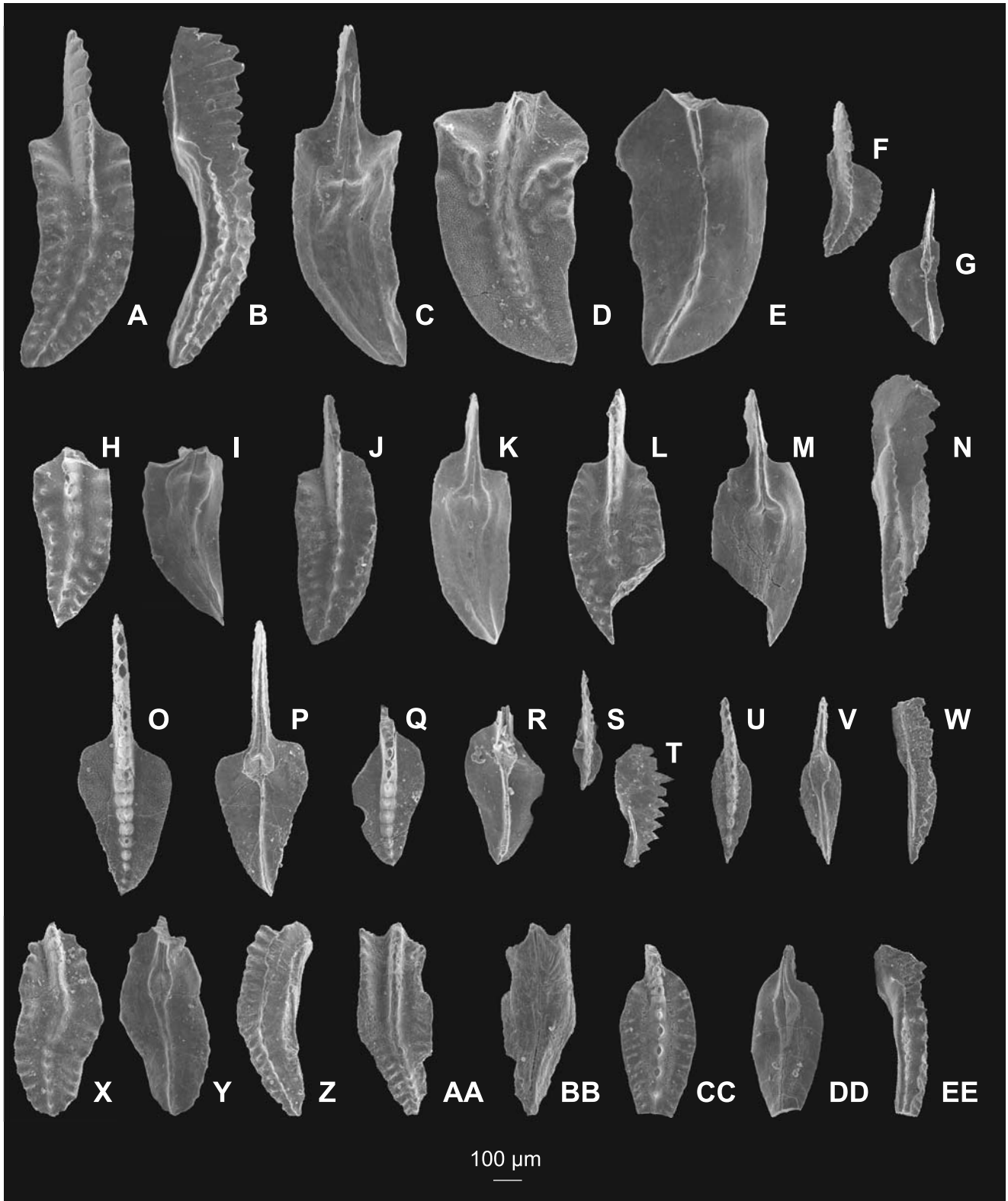
Fig. 7. Selected conodont elements ( P_1 ) of genus Polygnathus from the Kule section
