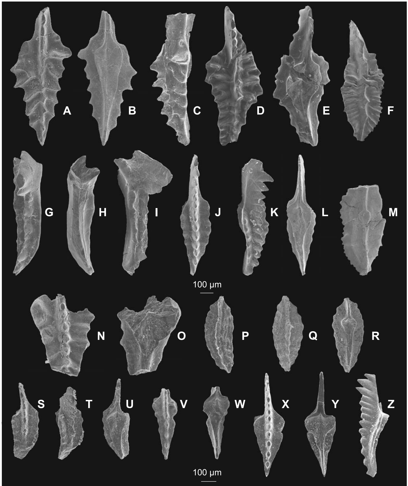
Fig. 8. Selected conodont elements ( P_1 ) of the genus Pseudopolygnathus from the Kule section
