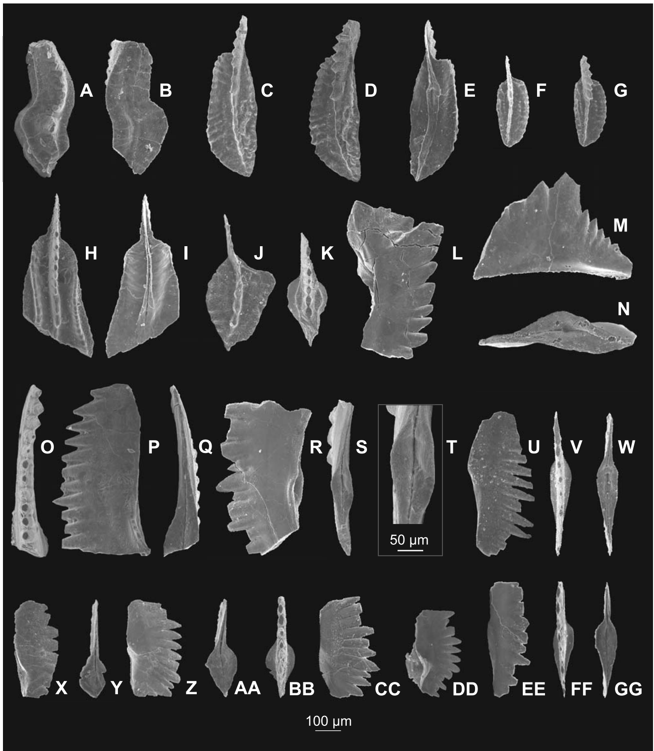
Fig. 6. Selected conodont elements ( P_1 ) from the Kule section
