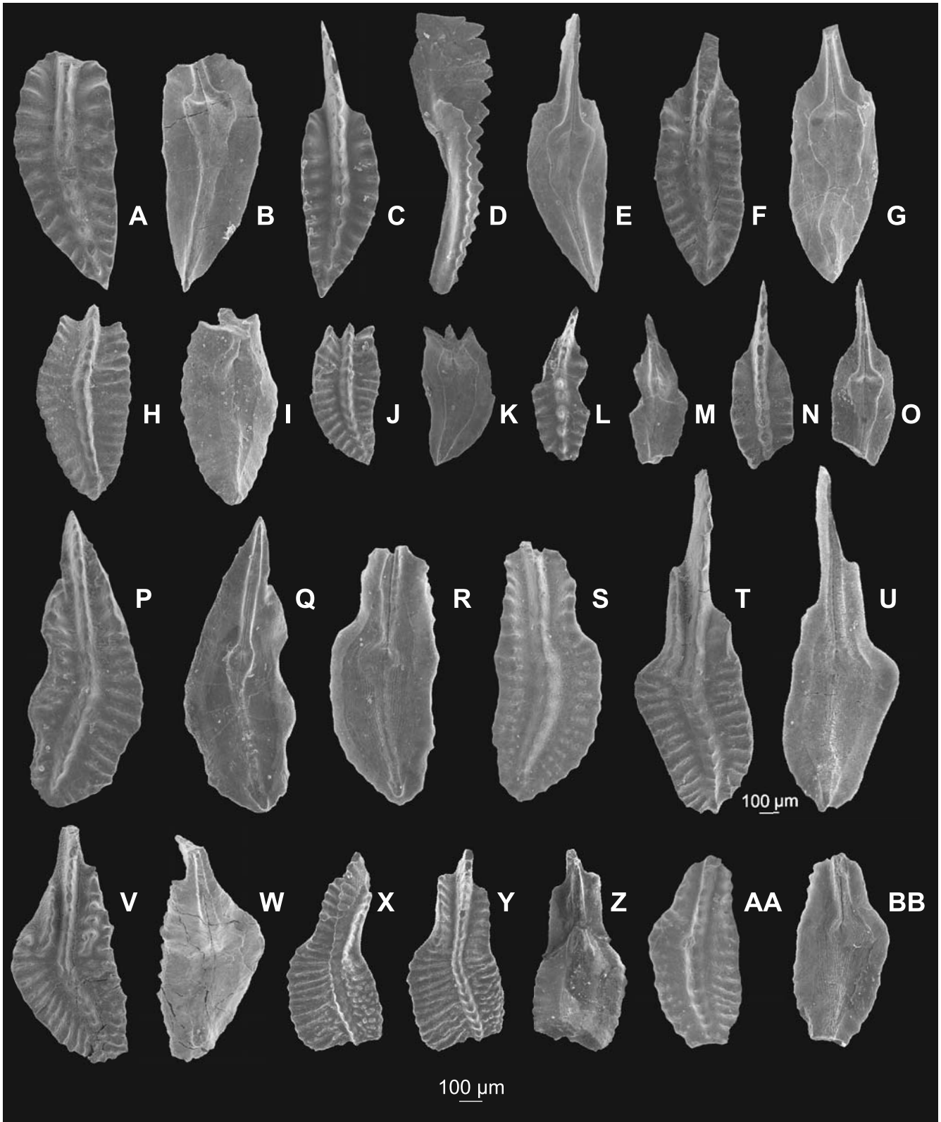
Fig. 5. Selected conodont elements ( P_1 ) of the genus Siphonodella from the Kule section
