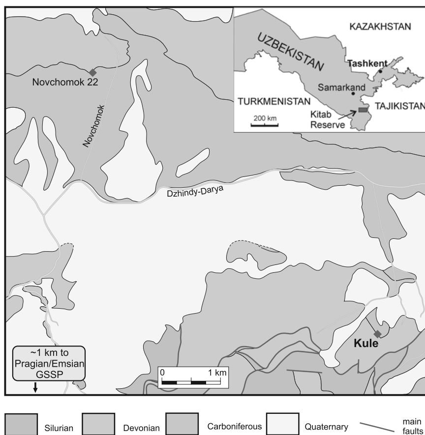
Fig. 1. Geological sketch-map showing the location of the section investigated, the inset map of Uzbekistan showing the location of the Kitab Reserve
