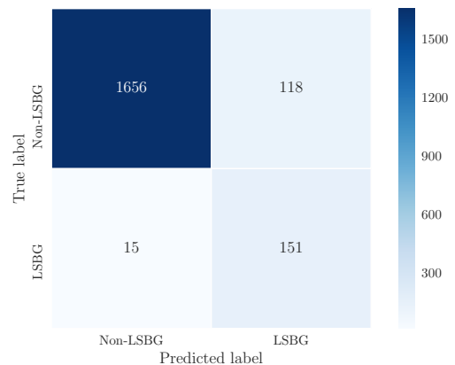
Figure 2. The confusion matrix of our final SVM classifier evaluated on the validation set. The quoted numbers correspond to the number of the validation instances (objects) based on their true and predicted label. The false-negative rate is \sim 9\% .
