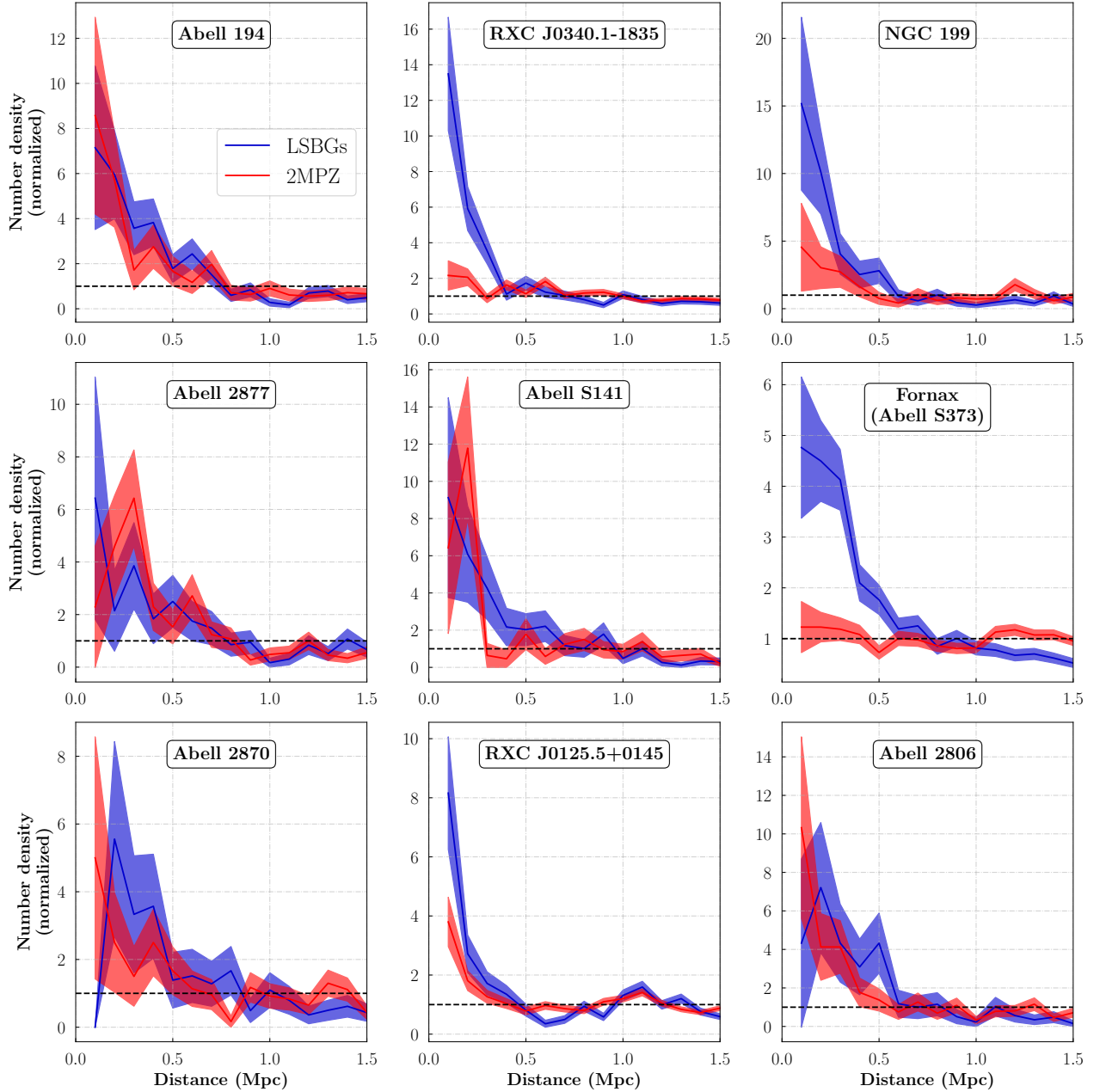
Figure 13. Normalized radial profiles of the distribution of LSB galaxies (blue) and galaxies from the 2MPZ catalog (red) around the associations of the most prominent LSB overdensity peaks, presented in Table 2. We have assumed that all galaxies that are within a radius that corresponds to a physical scale of 1.5 Mpc at the distance of the association belong to that association. The normalization constant corresponds to the mean number density of galaxies within the 1.5 Mpc radius.
