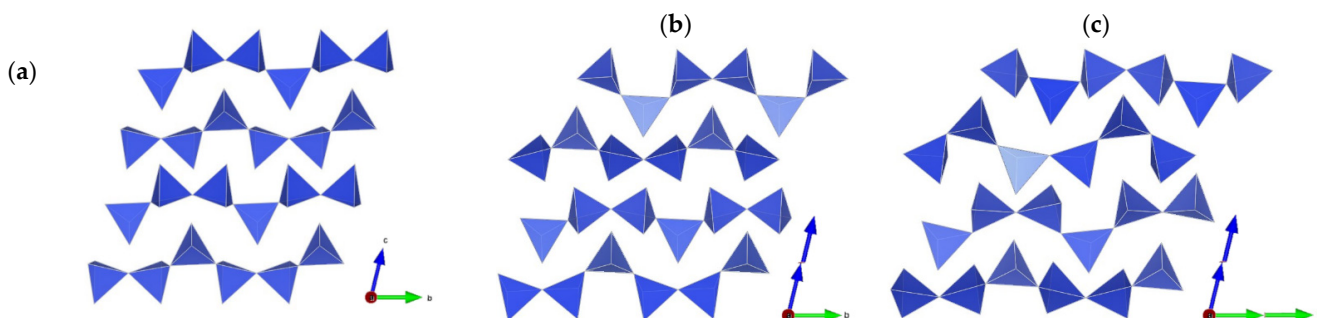
Figure 4. Phase transitions from (a) wollastonite-I (b) wollastonite-II and (c) wollastonite-III. The representations of the structure are realized using the program VESTA [17]; a axis points toward the reader, the green arrow is the b axis, while the blue arrow is the c axis. The blue and the green axis are doubled in (b,c) as it can be observed from the unit-cell parameters of the two polytypes (Table 3).
