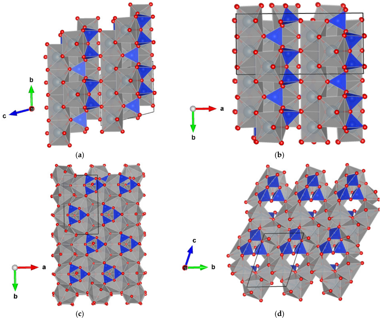
Figure 2. Crystal structure of (a) wollastonite, (b) wollastonite-2M, (c) pseudowollastonite, and (d) breyite. The representations of the structure are realized using the program VESTA [17]. Small red spheres are oxygens, (\text{SiO}_4)^{2-} are blue tetrahedra and grey polygons are Ca cation sites. Black solid lines represent the dimension of the unit cell.
