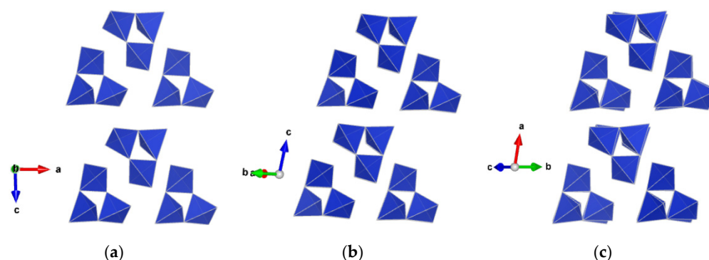
Figure 6. Phase transitions from (a) CaSiO 3 -walstromite-I (b) CaSiO 3 -walstromite-II and (c) CaSiO 3 -walstromite-III. The representations of the structure are realized using the program VESTA [17]; a axis is red, the green arrow is the b axis, while the blue arrow is the c axis.
