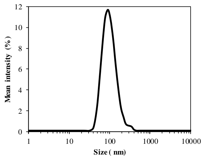
Figure S1: Example of DLS characterization of liposome suspensions after extrusion. In all cases, only one population of nano-vesicles with a narrow size distribution was found.
