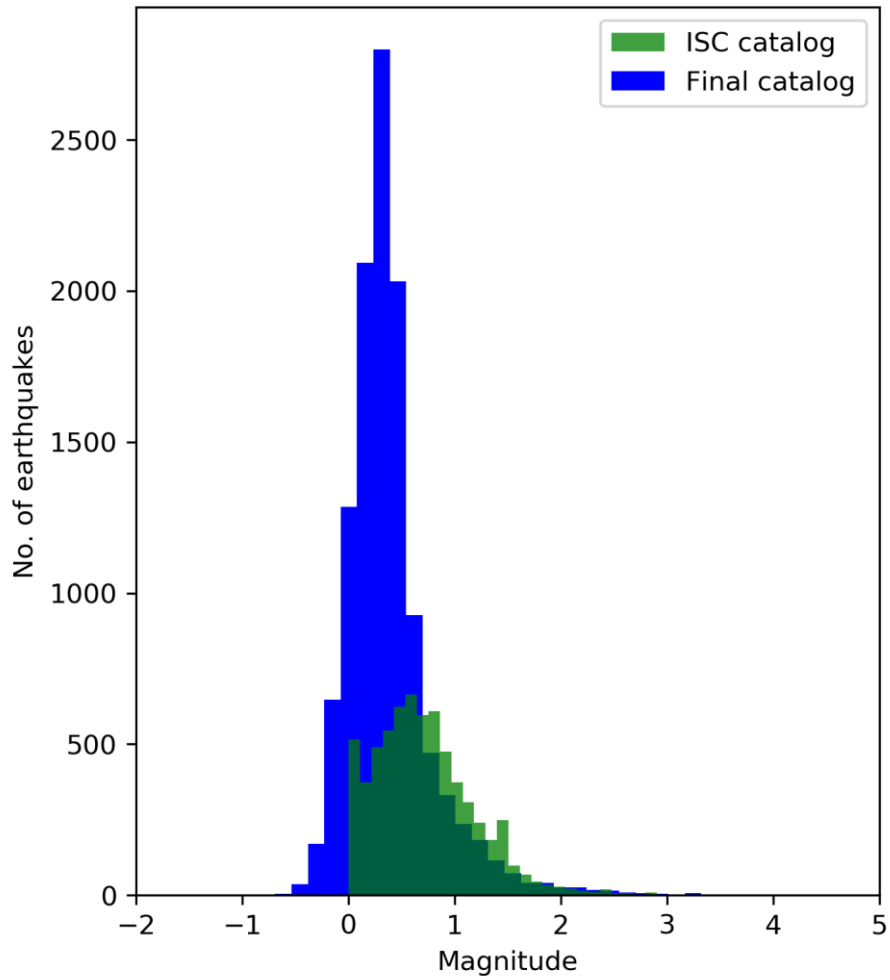
Figure S 2: Magnitude of completeness of the two catalogues. The magnitude of completeness of ISC catalogue is 0.9. The magnitude of completeness for final catalogue was lowered to -0.1 mainly due to the addition of low magnitude swarm events and missed earthquake activity along Ravne fault.
