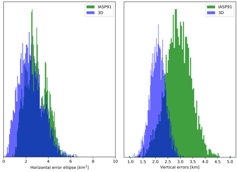
Figure S 5: Left figure represents horizontal errors of earthquakes located using IASP91 (green) model and 3D velocity model (blue). As observed in the figure, the horizontal errors do not change drastically. Right figure shows vertical errors using IASP91 model (green) and 3D model (blue). We observe lowering of the errors after relocation.
