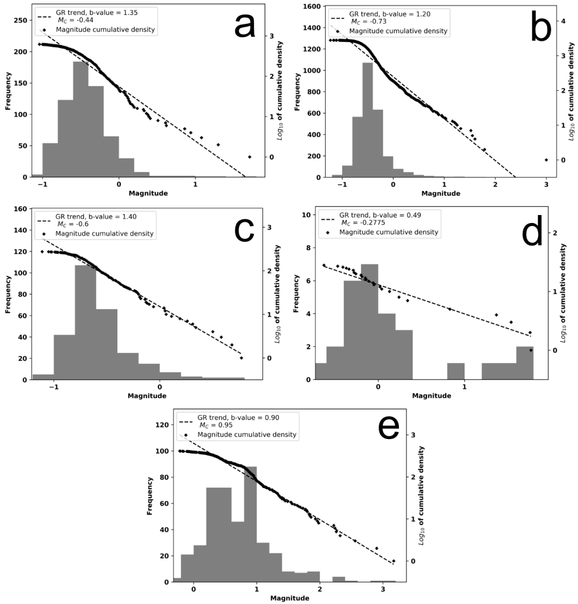
Figure S 7: Magnitude of completeness for the individual swarms observed along the active faults of western Slovenia. a) Vipava swarm 2006, b) Postojna swarm 2010, c) Selce swarm 2017, d) Ilirska Bistrica swarm 2017 and e) Rijeka swarm 2017.
