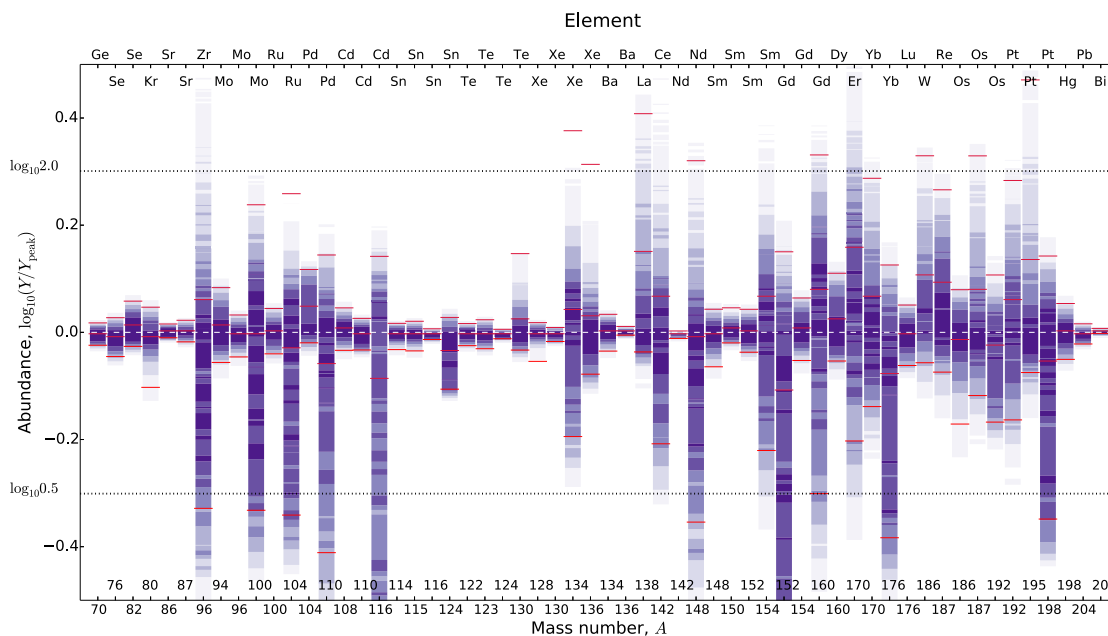
Figure 9. Total production uncertainties in the final s -process abundances obtained with the trajectory described in the previous section for the TP phase. The colour shading denotes the probabilistic frequency and the 90 per cent probability intervals up and down are marked for each nuclide with the red lines. The final abundances are normalized by the final abundance at the peak of the distribution. Horizontal dotted lines indicate a factor of 2 uncertainties.
