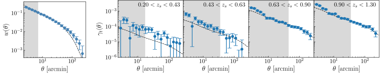
Figure 3. The angular galaxy clustering (left) and tangential shear data (right) from Lee et al. (2019) and Lee et al. (2021). The signals are measured with the D MASS (lenses) and DES Y1 METACALIBRATION (sources) catalogs. The dashed lines are the best-fitting MG predictions from the combination of the baseline case (D MASS 3x2pt + CMASS RSD/BAO) and Planck data. The shaded regions are discarded in the analysis to exclude the small scales where the phenomenological parametrization is not valid. The remaining data points are 16 points for w(\theta) and 38 points for \gamma_t(\theta) .
