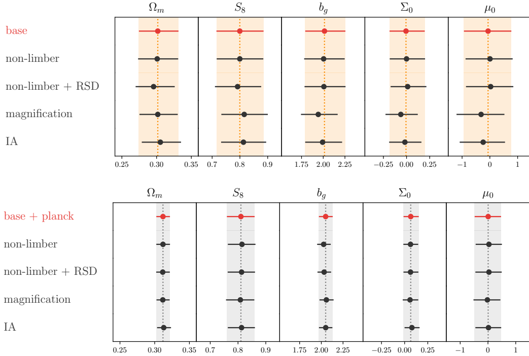
Figure 5. Marginalized 1D posterior constraints on \Omega_m , S_8 , b , \Sigma_0 , \mu_0 obtained from DMASS 3x2pt + CMASS RSD/BAO (baseline; top) and DMASS 3x2pt + CMASS RSD/BAO + Planck (bottom). The different rows correspond to the different systematics injected in each of the simulated data vectors. The systematics tested here are detailed in Section 5. These data vectors are analyzed by the fiducial pipeline to test the impact of systematics associated with each data vector on the parameter constraints. For all cases, the posteriors for these cosmological parameters remain well within 1\sigma of the fiducial constraints.
