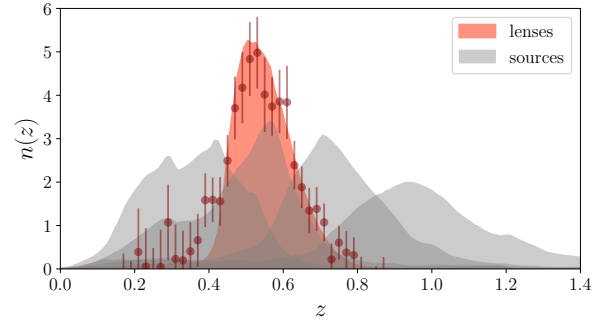
Figure 2. The spectroscopic redshift distribution of BOSS CMASS (red shaded) and the photometric redshift distributions of METACALIBRATION (grey shaded). The maroon color points with error bars show the redshift distribution of DMASS computed by cross-correlating the sample with the DES Y1 REDMAGIC sample. As the redshift distributions of CMASS and DMASS show good consistency, we use the redshift distribution of CMASS as the true redshift distribution for a theoretical prediction for DMASS. The source sample, METACALIBRATION is divided into 4 tomographic bins ( 0.2 < z_s < 0.43 , 0.43 < z_s < 0.63 , 0.63 < z_s < 0.90 and 0.90 < z_s < 1.30 ) using the BPZ photometric redshift code.
