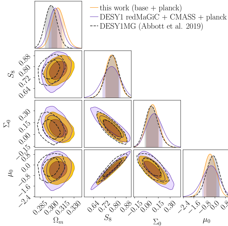
Figure 8. Constraints from this work (baseline+ Planck ; orange), DESY1 REDMAGiC 3x2pt + CMASS RSD/BAO + Planck (purple), and the published constraints of the DES Y1 MG analysis (black-dashed) (Abbott et al. 2019). Compared to the case with REDMAGiC (purple), using DMASS (orange) improves the MG constraints by 29% for \mu_0 and 21% for \Sigma_0 with the same external data sets. The DMASS case is even comparable to that of DESY1MG (black-dashed) despite the lack of the external data sets. The shift of \Omega_m in DESY1MG is caused by the SNe Ia data favoring low \Omega_m . Overall, the constraints in the three cases are consistent.
